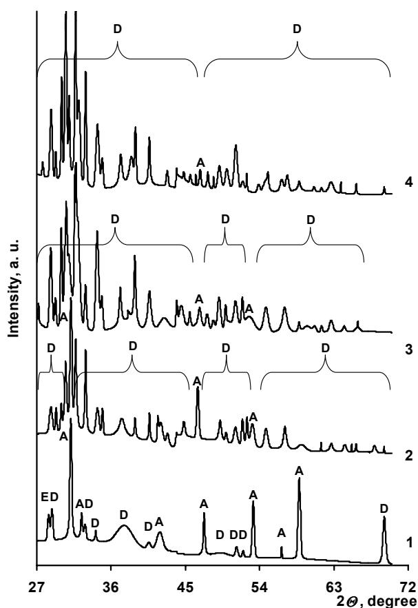
Fig. 5. X-ray diffraction patterns of thallium sulphide layers in the surface of PA. PA initially treated with a solution of \text{H}_2\text{S}_{12}\text{O}_6 at 30 °C different time and then with a \text{Ti(I)} salt solution at 80 °C for 10 min. Sulfuration time, h: 1 – 0.5; 2 – 1.0; 3 – 3.0; 4 – 6.0. A – \alpha\text{-TiS} [30–1331]; D – orthorhombic \text{Ti}_2\text{S}_5 [71–358]; E – \beta\text{-Ti}_4\text{S}_3 [43–1067]
