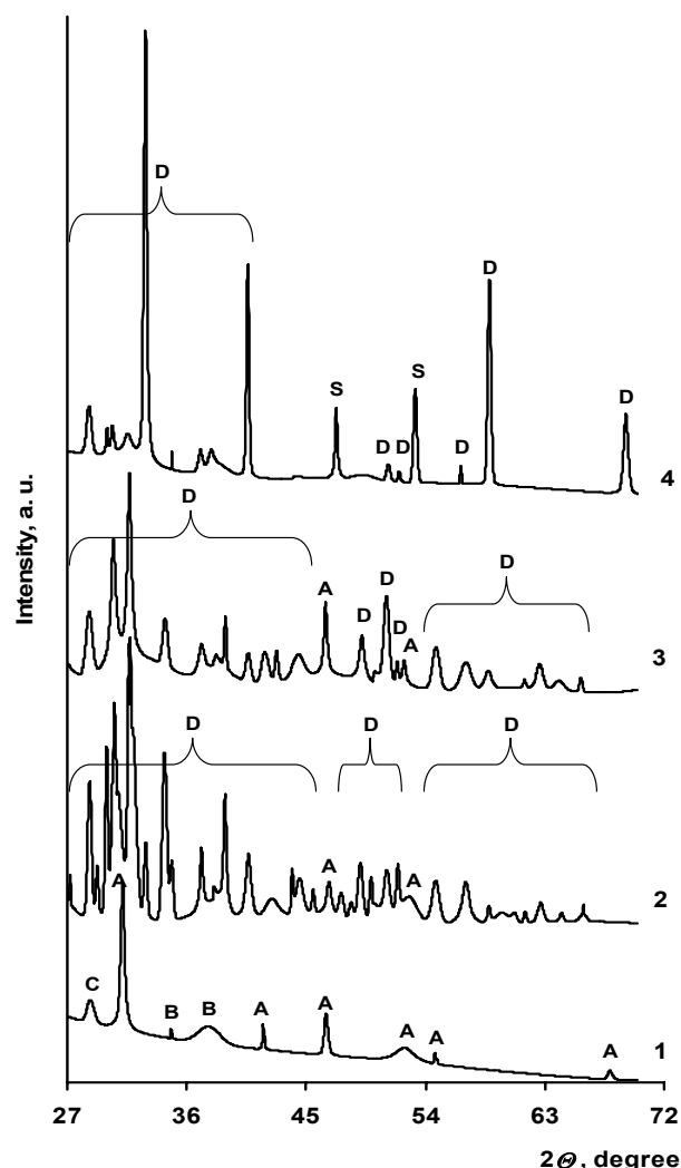
Fig. 6. X-ray diffraction patterns of thallium sulphide layers in the surface of PA. PA initially treated with a solution of \text{H}_2\text{S}_{12}\text{O}_6 for 3 h at different temperature and then with a \text{Ti(I)} salt solution at 80 °C for 10 min. Temperature, °C: 1 – 20; 2 – 30; 3 – 40; 4 – 50. A – \alpha\text{-TiS} [30–1331], B – tetragonal \text{Ti}_2\text{S}_2 [82–2050], C – monoclinic \text{TiS} [82–2050], D – orthorhombic \text{Ti}_2\text{S}_5 [71–358], S – elemental sulfur S [24–1206]
