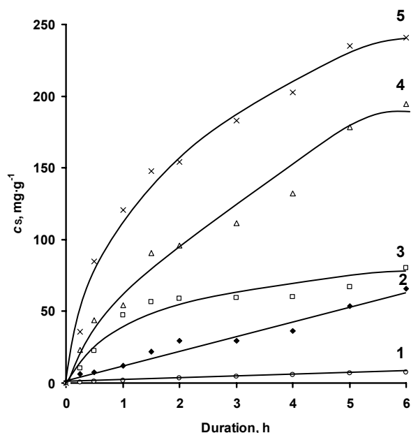
Fig. 3. Change of sulfur concentration in PA with time during its treatment with acidified ( 0.1 \text{ mol} \cdot \text{dm}^{-3} \text{HCl} ) 0.1 \text{ mol} \cdot \text{dm}^{-3} \text{K}_2\text{S}_5\text{O}_6 solution at 20^\circ\text{C} (1) and with 0.002 \text{ mol} \cdot \text{dm}^{-3} solution of \text{H}_2\text{S}_{12}\text{O}_6 at different temperatures. Temperature, ^\circ\text{C} : 2 – 20; 3 – 30; 4 – 40; 5 – 50
