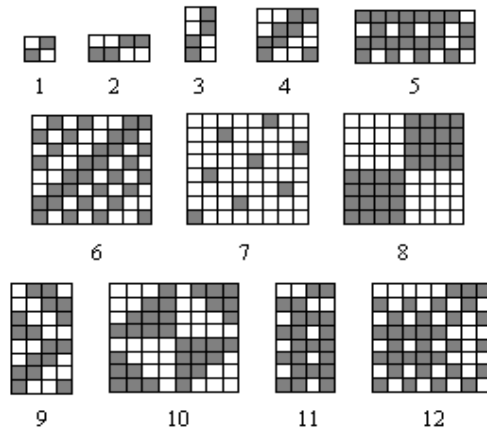
Fig. 1. The weaves using for experiment: 1 – plain weave; 2 – weft rib; 3 – warp rib; 4 – twill 2/2; 5 – weft direction Bedford cord; 6 – fancy twill; 7 – sateen; 8 – basket weave; 9 – broken twill; 10 – crape weave; 11 – warp direction Bedford cord; 12 – mock leno
