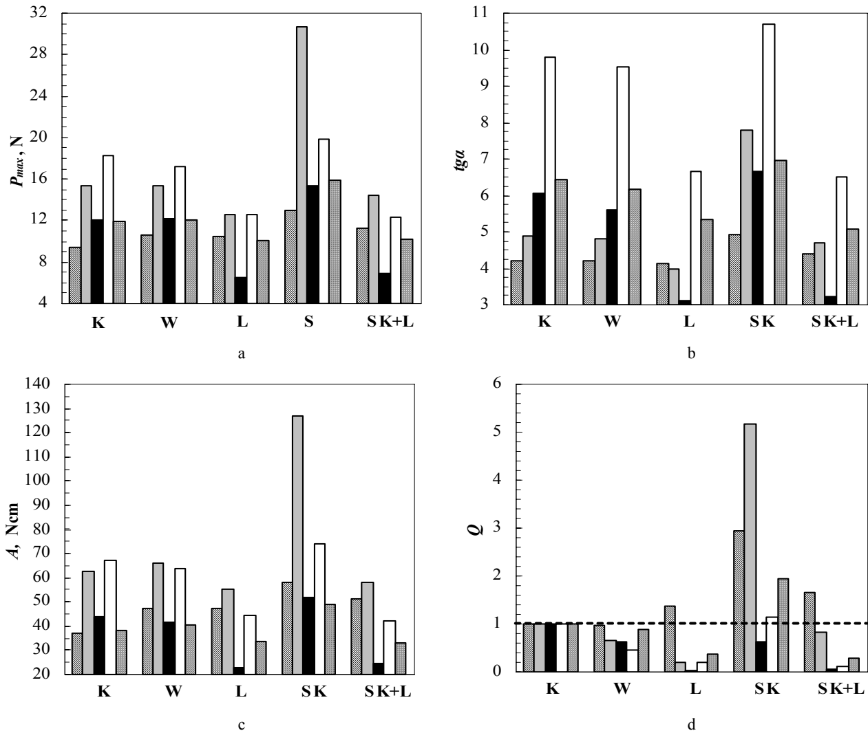
Fig. 3. The diagrams of the parameters P_{max} (a), tga (b), A (c) and Q (d) during treatment of the test samples (■ -T11 ■ -T12 ■ -T13 □ -T14 ■ -T15, 1 Table)
