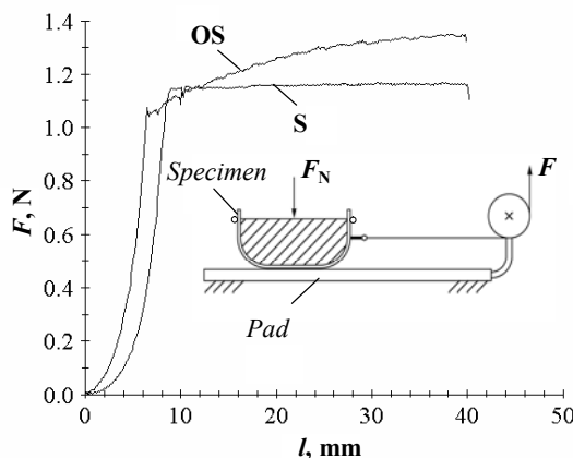
Fig. 1. Friction curves for fabric T13 to a glass surface (S) and organic glass surface (OS)
