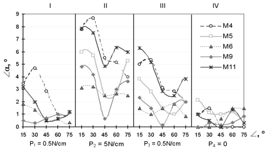
Fig. 7. The influence of loading conditions (I, II, III and IV stages) and cut direction of specimen upon the shear angle \alpha_n
