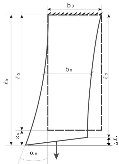
Fig. 3. Specimen's shape after stretching and measured parameters
