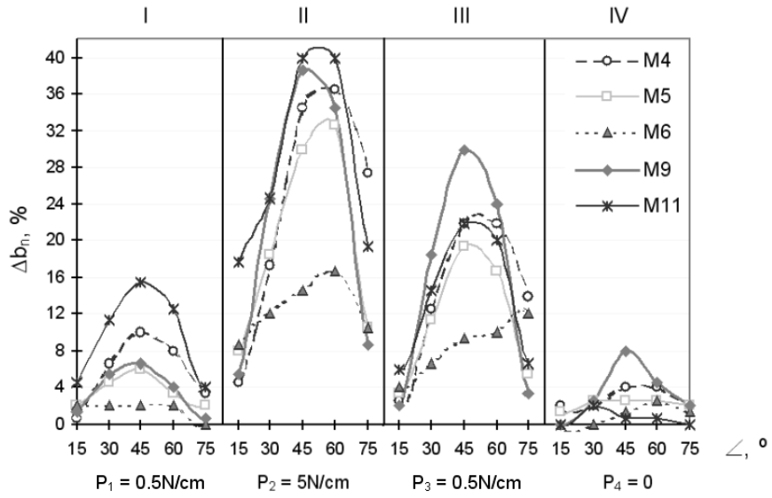
Fig. 5. The influence of loading conditions (I, II, III and IV stages) and cut directions of specimen upon the relative decrease of specimen's width \Delta b_n (%)
