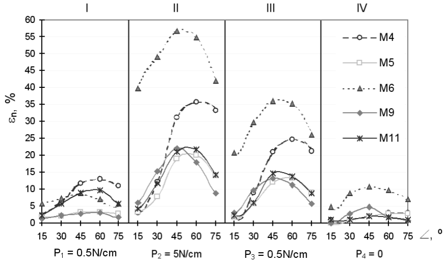
Fig. 4. The influence of loading conditions (I, II, III and IV stages) and cut directions of specimen upon the elongation \varepsilon_n
