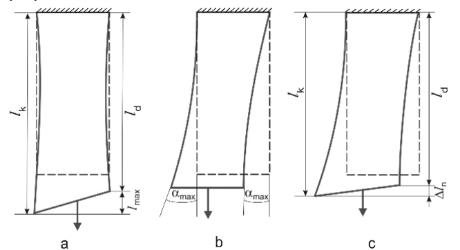
Fig. 8. Different types of textile fabrics non-uniformity
