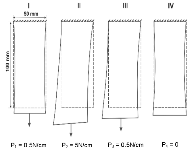
Fig. 2. Four stages of the experiment
