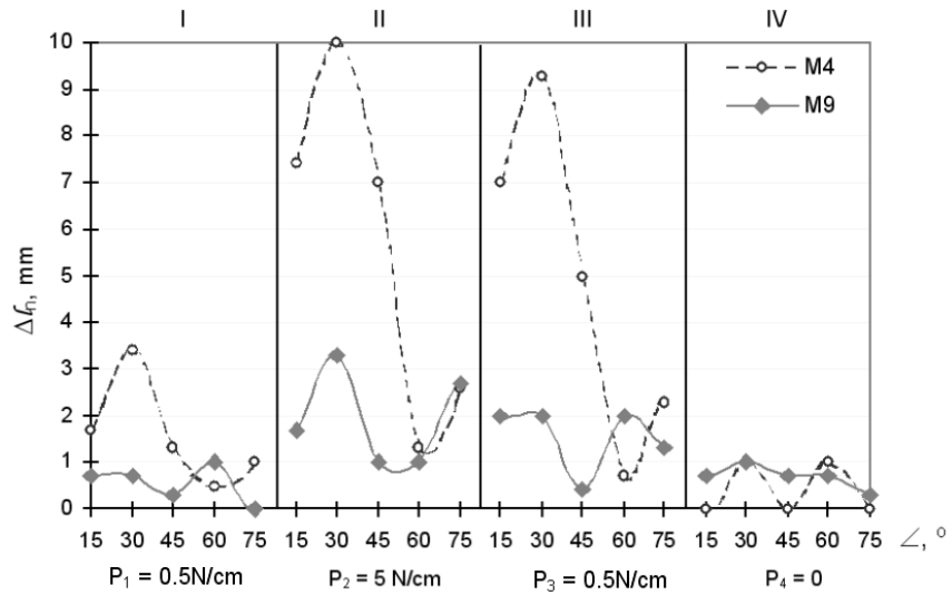
Fig. 6. The influence of loading conditions (I, II, III and IV stages) and cut direction of specimen upon the difference of specimen's edges length \Delta l_n
