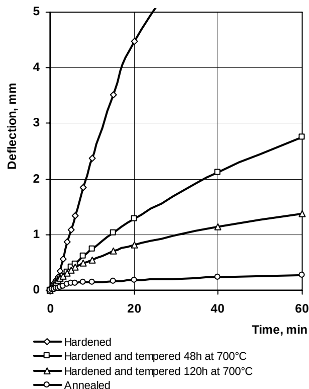
Fig. 5. Dependence of steel 12XH3A plasticity on structural state during tempering at 650 °C temperature. Bending stress 90 N/mm 2
