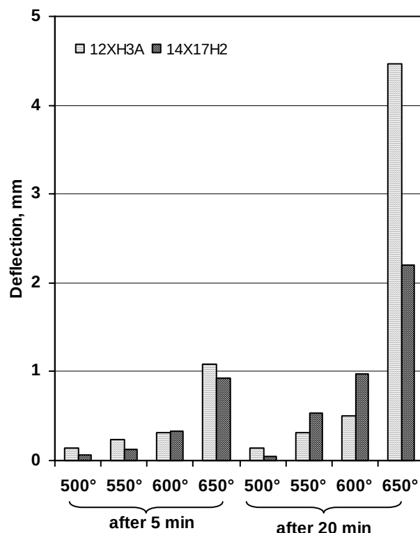
Fig. 3. Comparison of plastic deflection of steel 14X17H2 and steel 12XH3A specimens in process of bending experiments at various tempering temperatures: after 5 min of bending and after 20 min of bending. Bending stress 90 N/mm 2
