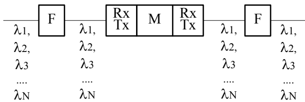
Fig. 2. Structure of M_1 node
