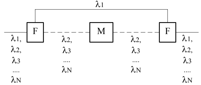
Fig. 4. Structure of M_3 node
