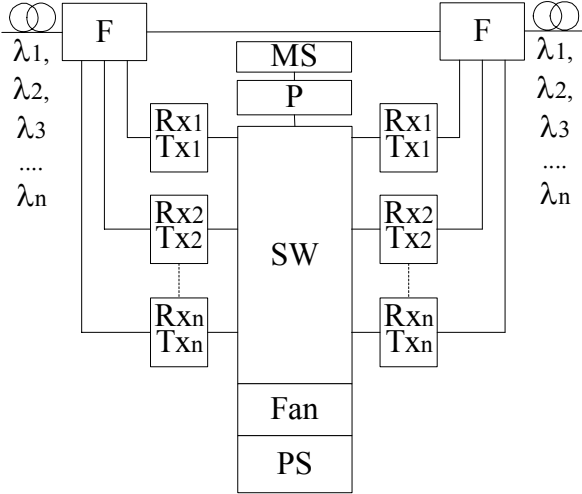
Fig. 1. Structure of an optical network
