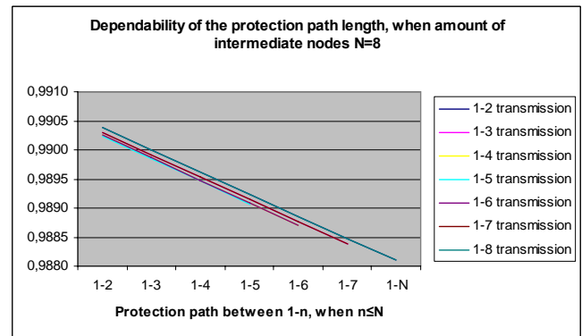
Fig. 7. Dependability of the protection path length
