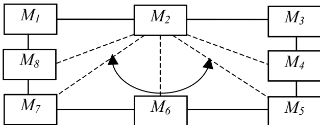
Fig. 6. One-channel ring network topology composed of 8 nodes
