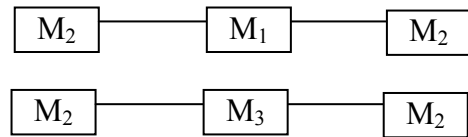
Fig. 5. Availability estimation structure of a network
