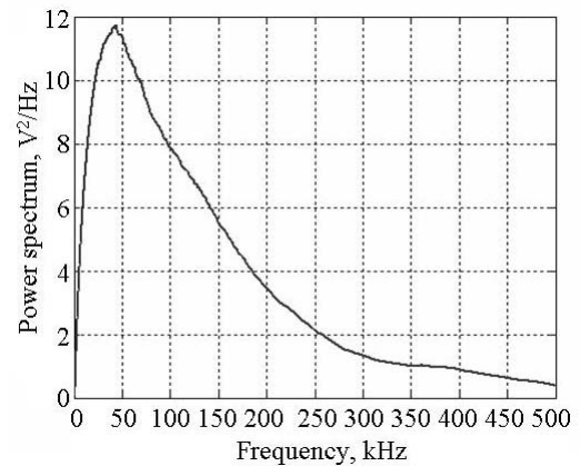
Fig. 2. Calculation of certain MBN spectrum in specimen (Calibration procedure): c = a / b ; a – MBN signal spectrum without calibration ( FT[U_B(t)] ); b – frequency response of a measurement channel ( K_{HU}(j\omega) ); c – MBN signal spectrum after calibration ( S_H(j\omega) )
