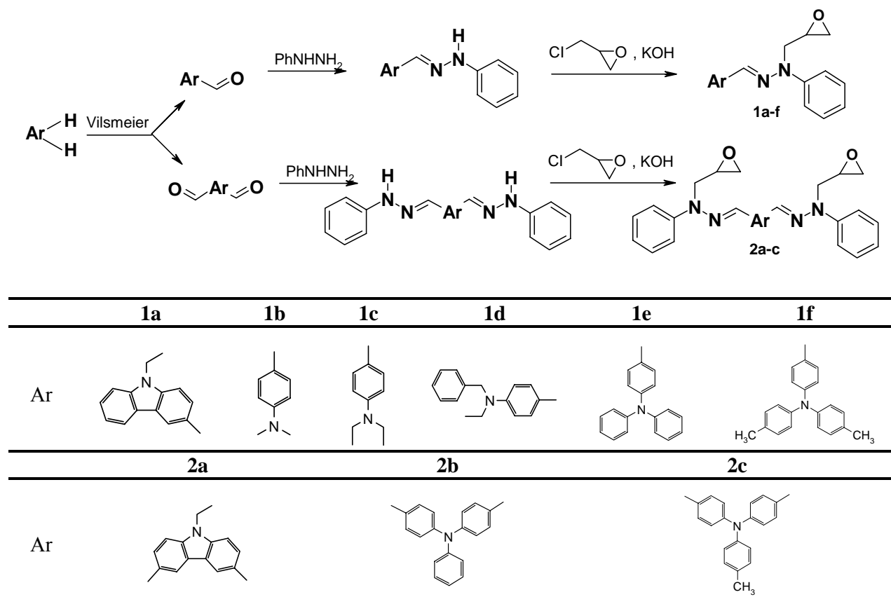
Scheme 1. Synthetic route to the epoxides 1a-i containing hydrazone moieties
