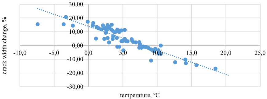
Fig. 7. The crack width change relationship with temperature in crack-gauges B when wind speed is above 10 m/s
