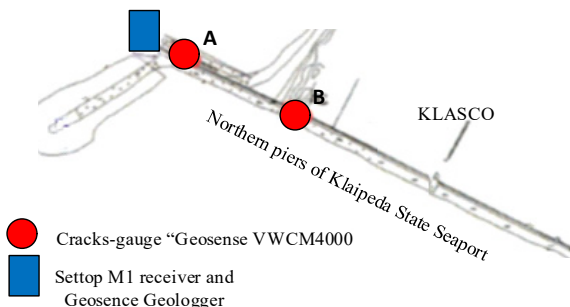
Fig. 3. The location places of crack-gauges
