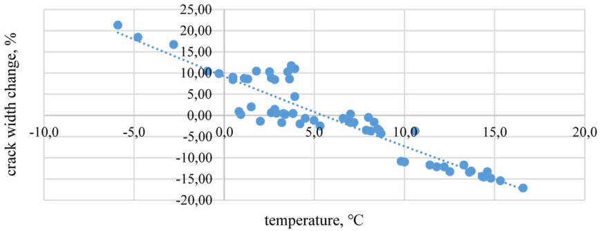
Fig. 4. The crack width change relationship with temperature in crack-gauges A when wind speed is under 10 m/s
