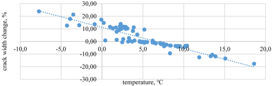
Fig. 5. The crack width change relationship with temperature in crack-gauges A when wind speed is above 10 m/s
