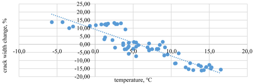
Fig. 6. The crack width change relationship with temperature in crack-gauges B when wind speed is under 10 m/s
