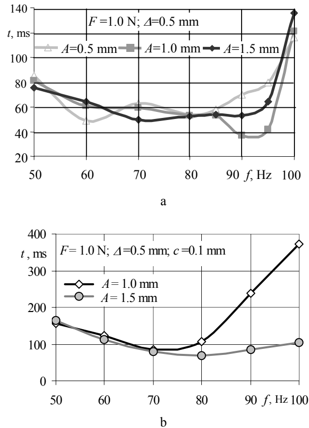
Fig. 6 Dependence of alignment duration t on excitation frequency f , under different excitation amplitudes A : a – for the parts of circular cross-section; b – for the parts of rectangular cross-section (where c – joint clearance)
