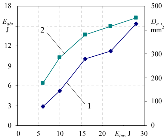
Fig. 9 Absorbed energy and damage area plotted against the impact energy of woven glass-fiber-reinforced composites. The exclusion line: 1 - absorbed energy; 2 - damage area
