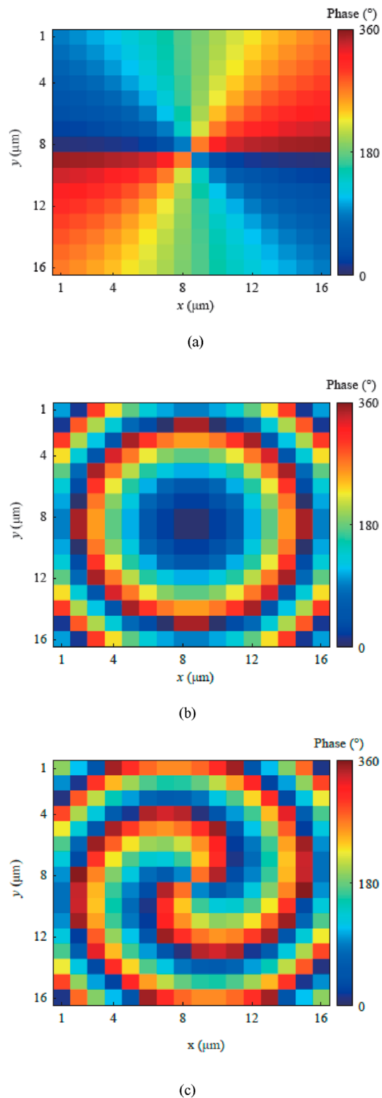
FIGURE 4 Phase distribution determination of metasurface. (a) Vortex phase \varphi_1 ; (b) focus phase \varphi_2 ; (c) total compensation phase \varphi_{tot} .
