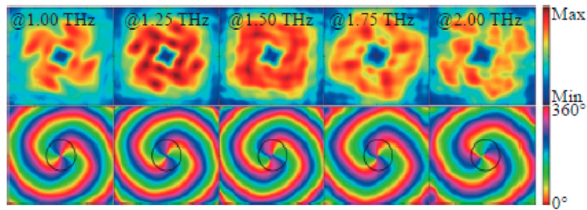
FIGURE 7 Amplitude and phase evaluation of vortex waves at l = -2 (near-field).
