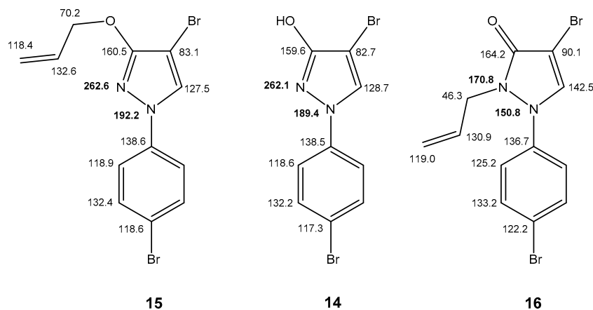
Figure 7. ^1\text{H} (in italics), ^{13}\text{C} and ^{15}\text{N} (in bold) NMR chemical shifts of 14 and its “fixed” derivatives 15 and 16 (in \text{CDCl}_3 ).
