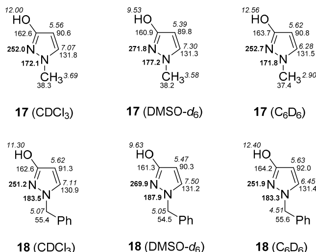
Figure 8. Crucial ^1\text{H} (in italics), ^{13}\text{C} , and ^{15}\text{N} (in bold) NMR chemical shifts of 1-methyl-1 H -pyrazol-3-ol ( 17 ) and 1-benzyl-1 H -pyrazol-3-ol ( 18 ) in \text{CDCl}_3 , \text{DMSO-}d_6 , and \text{C}_6\text{D}_6 solution.
