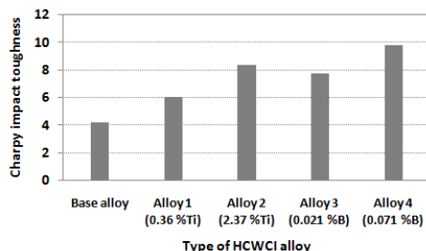
Figure 4. The influence of the individual addition of Ti and B on the Charpy V notch impact toughness of tested as-cast HCWCIs
