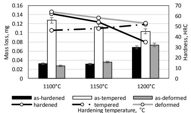
Fig. 5: Wear and hardness results of three test batches.
