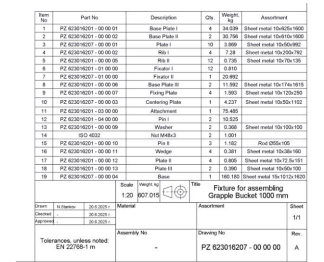
Fig. 20. Drawing of the fixture for assembling a 1000 mm grapple bucket.
