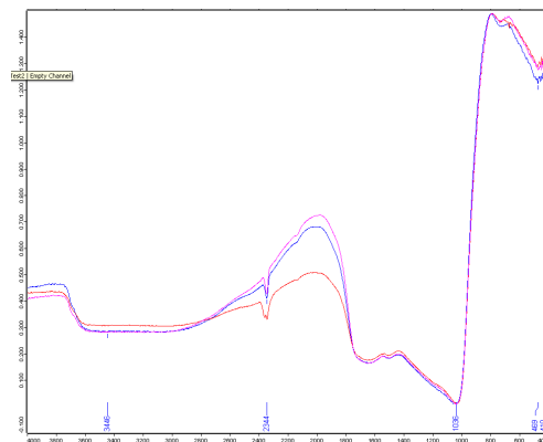
Fig. 5. FTIR transmittance spectra (a.u.) of three nanoporous aluminium oxide membranes for wavenumber of 4000-400 cm -1
