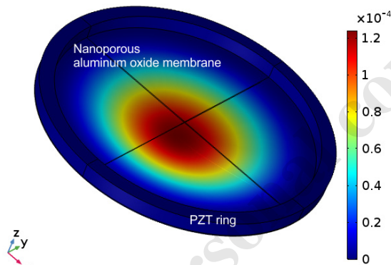
Fig. 6. Vibration of nanoporous aluminum oxide membrane
