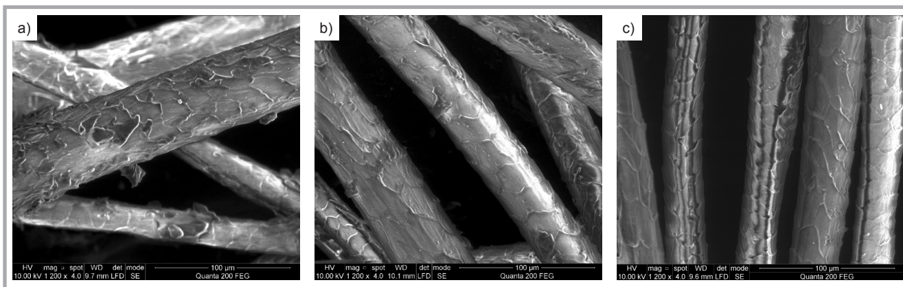
Figure 2. SEM photographs: a) native wool, b) wool treated 24 hours with \text{Ca}(\text{OH})_2 , c) wool treated 24 hours with \text{NaAlO}_2 (magnification: \sim 1200 times).
