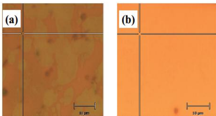
FIGURE 5.2 Optical images for (a) sample A, (b) sample B as deposited on copper foil
