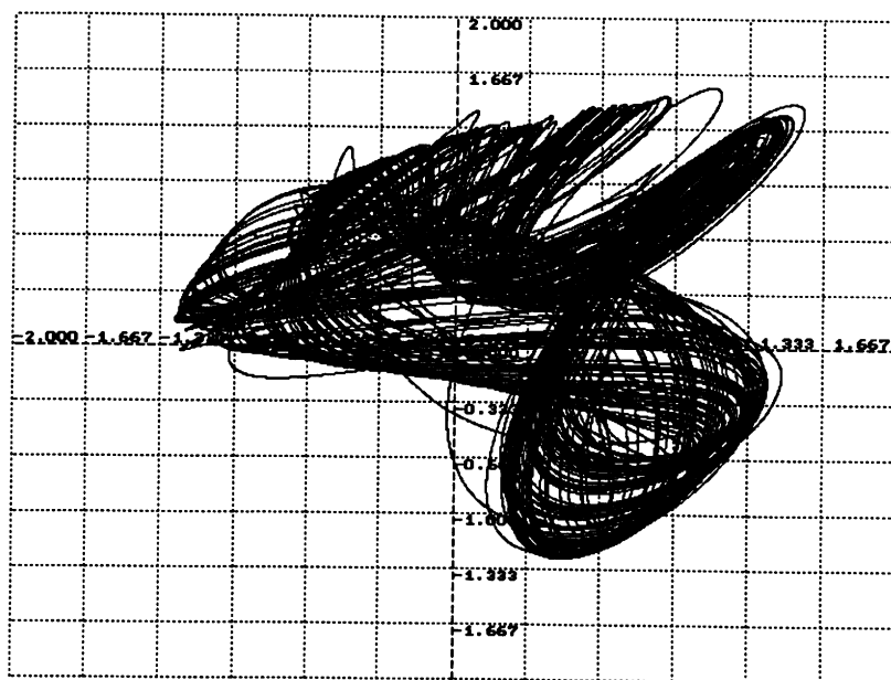
Fig. 3. The attractor of the same system as in Fig. 2. Here X axis stands for velocity u' , Y axis - for u' + p , here p - the length of the interval, p = \pi/4 .
