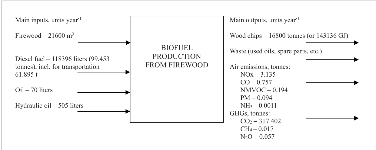
Fig. 3 Material and energy flows of wood chips production from firewood and transportation to combustion plant (-s), units year -1 (company’s data, 2015)
