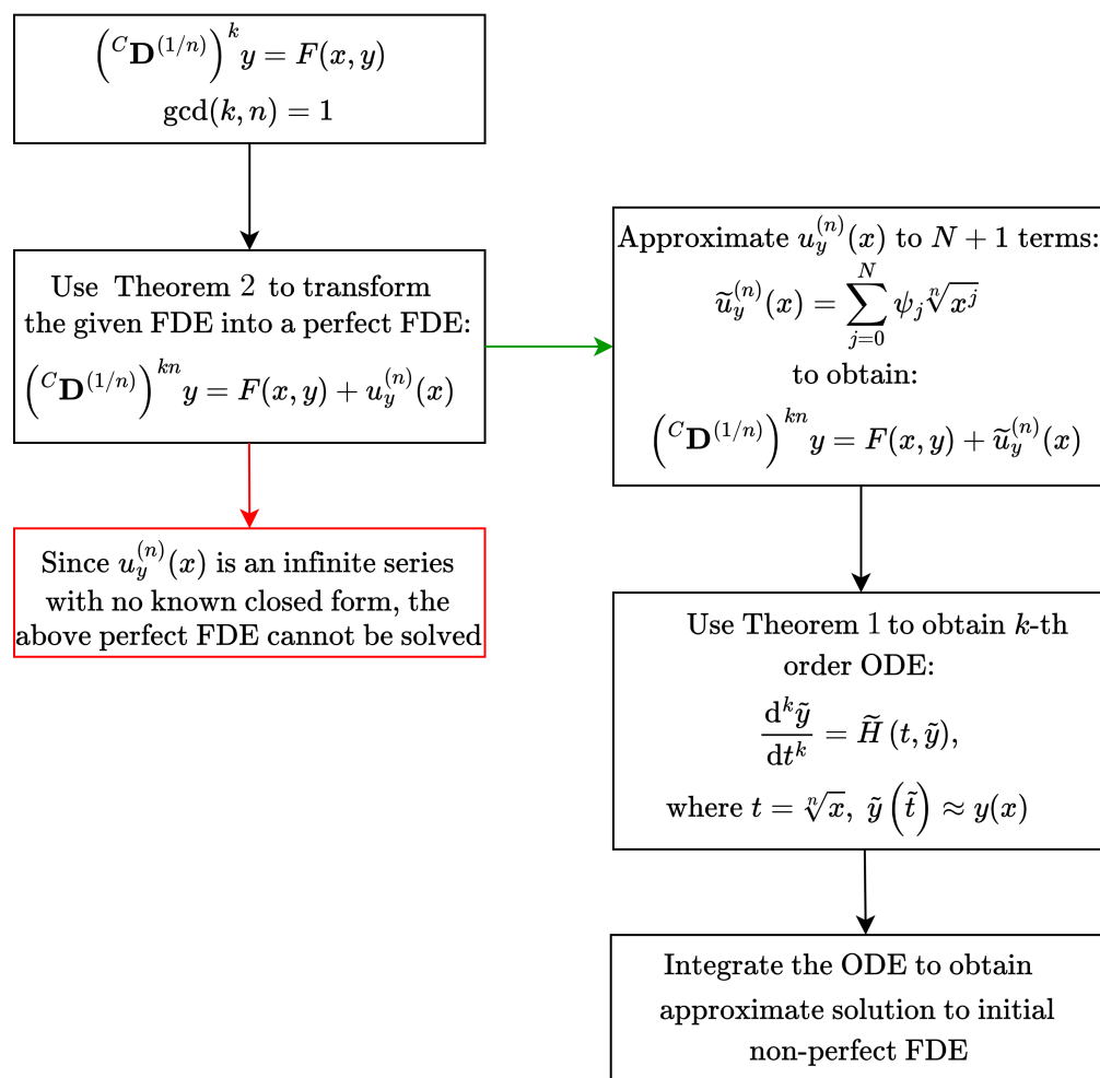
Figure 1. Schematic diagram of construction of solutions to FDEs of type ({}^C\mathbf{D}^{(1/n)})^k y = F(x, y) .
