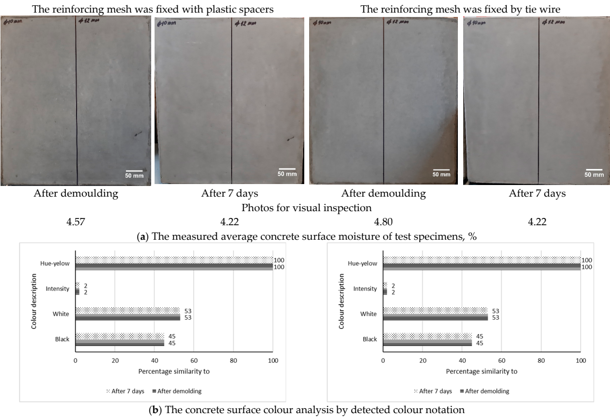
Figure 7. The concrete cover thickness is 35 mm (C-RS-1).
