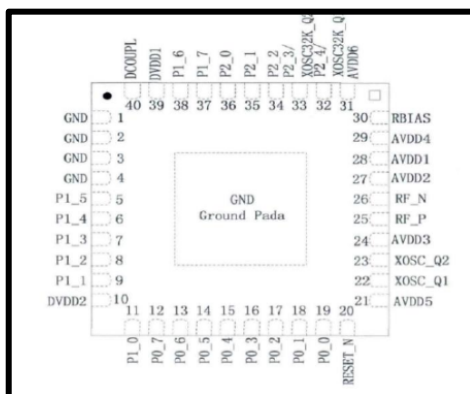
Figure 4: Functional diagram of the CC2530 connection sockets. Source: Du Yuhan. (2024). Research on Security System of Smart Home Based on ZigBee. International Journal of Computer Science and Information Technology , 4, 37-45.
