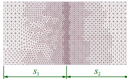
Figure 2. Mesh of a two-layer roll finite element model (flat, axisymmetric model)
