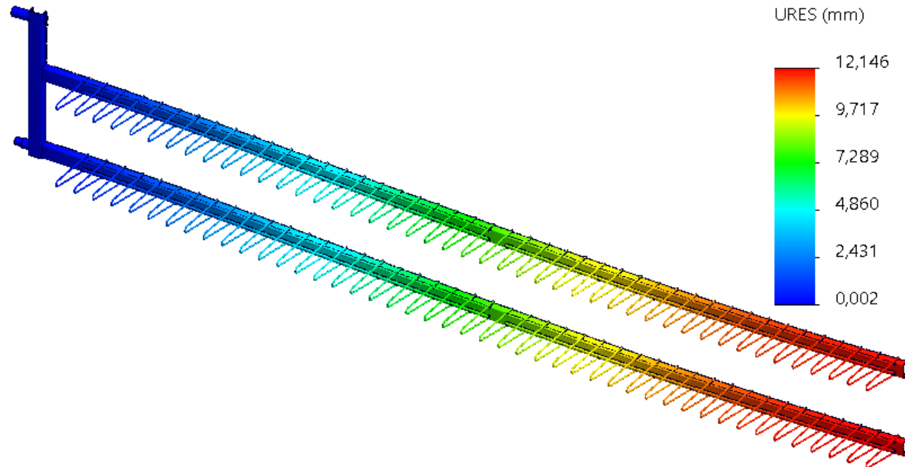
Figure 12. Distribution of deflections of hanger No 1
