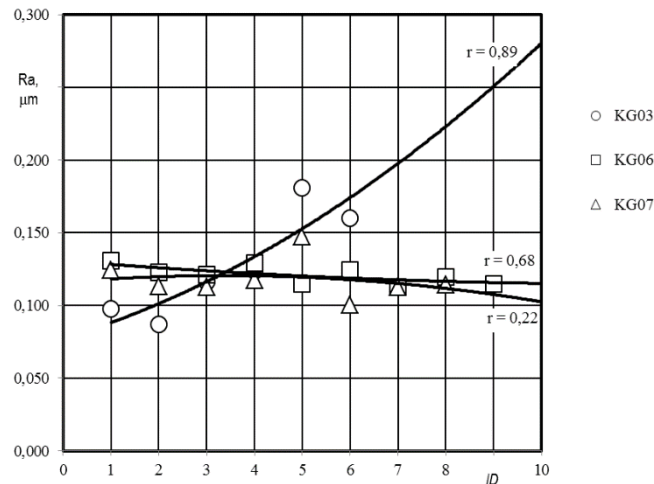
Figure 8. Variation with time of the bearing outer ring roughness parameter R_a using Pemco 10w40 engine oil for lubrication: bearing KG03 ( n = 500 \text{ rpm} ), bearing KG06 ( n = 750 \text{ rpm} ) and bearing KG07 ( n = 1000 \text{ rpm} )
