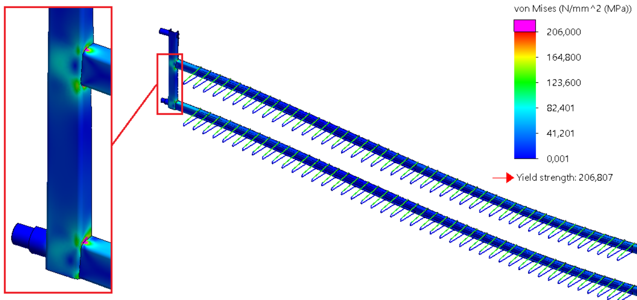
Figure 10. Stress distribution of hanger No 1
