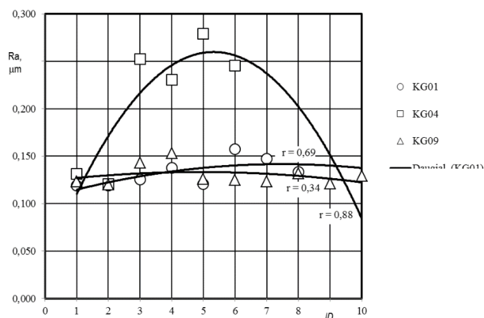
Figure 6. Variation with time of the roughness parameter R_a of the bearing outer ring working surface using Autol Top 2000 thick lubricant: bearing KG01 ( n = 250 rpm), bearing KG04 ( n = 750 rpm) and bearing KG09 ( n = 1000 rpm)
