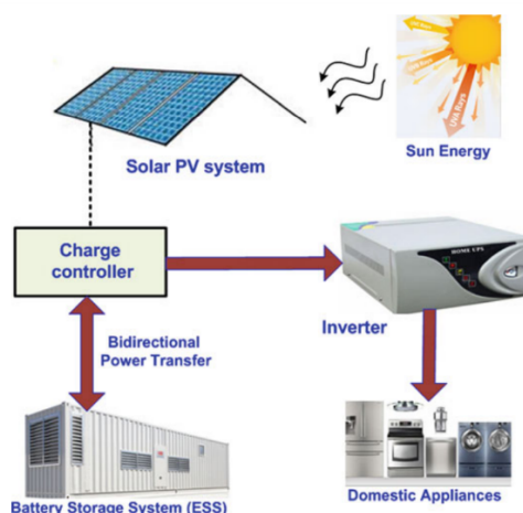
Figure 2. Off-grid solar power plant network
