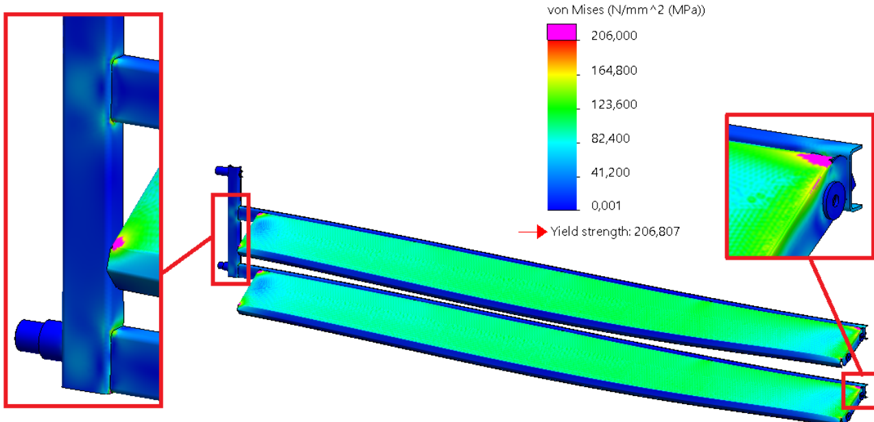
Figure 11. Stress distribution of hanger No 2
