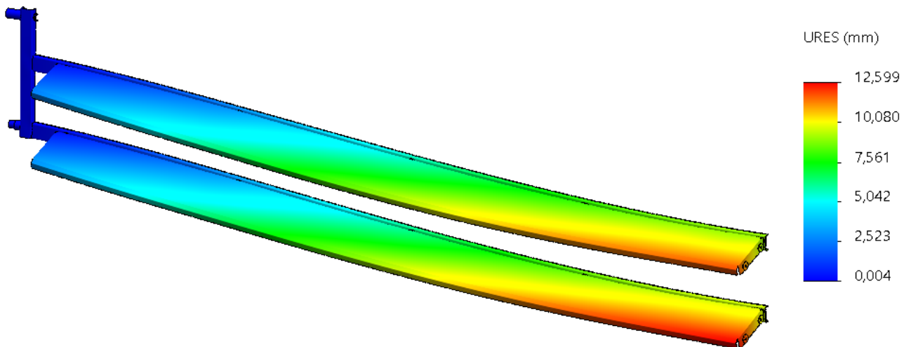
Figure 9. Distribution of deflections of hanger No 2
