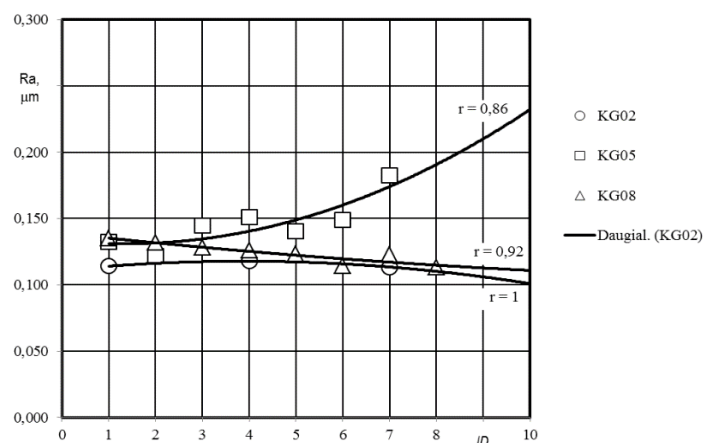
Figure 7. Variation with time of the roughness parameter R_a of the working surface of the outer ring of the bearing for lubrication with Pemco 80w-90 gear oil: bearing KG02 ( n = 500 rpm), bearing KG05 ( n = 750 rpm) and bearing KG08 ( n = 1000 rpm)
