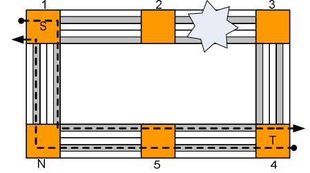
Fig. 8. 1+1 wavelength channel protection in the case of a failure on working path
