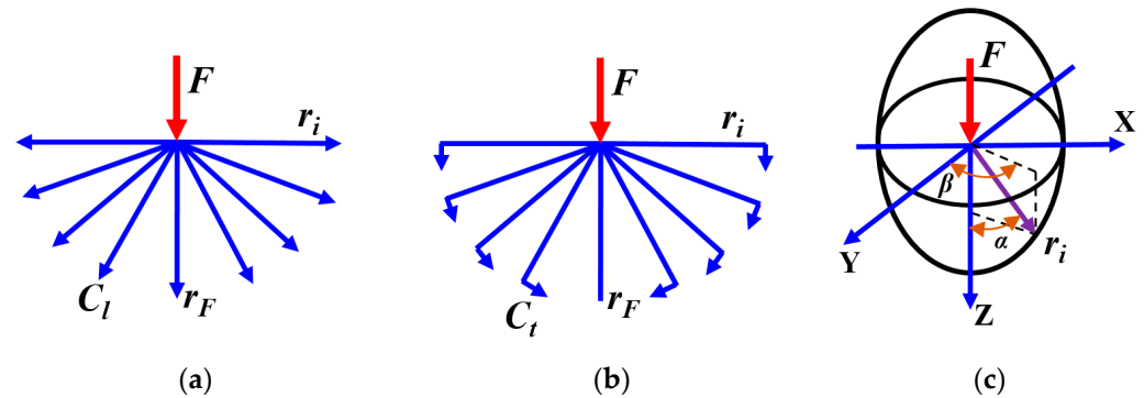
Figure 1. Directional movement under: (a) the longitudinal waves' action, (b) the transverse waves' action, (c) both waves' action.
