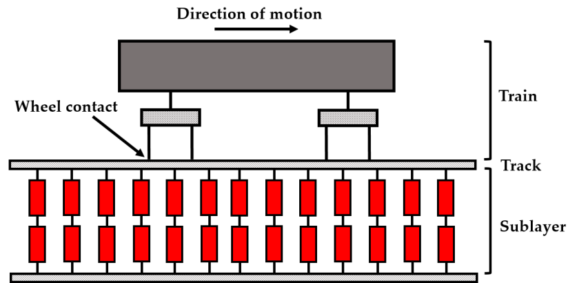
Figure 5. Schematic of the coupled system.
