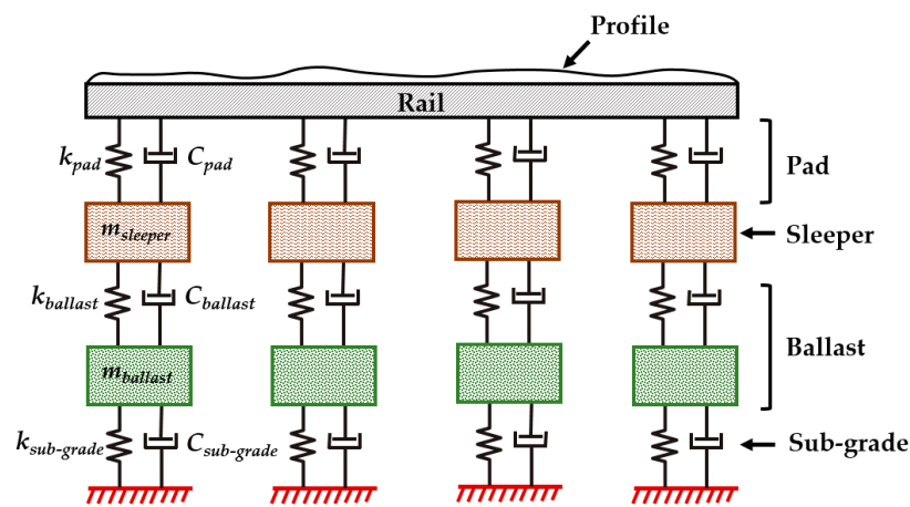
Figure 6. Track numerical model.
