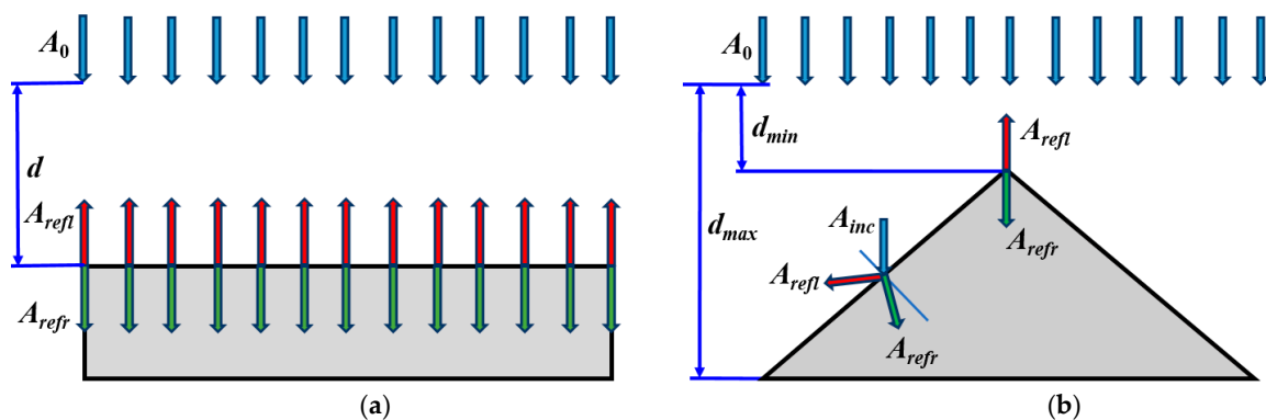
Figure 4. Changes in the parameters of the impact of the primary impulse A_0 when falling on: (a) rectangular object, (b) triangular object.
