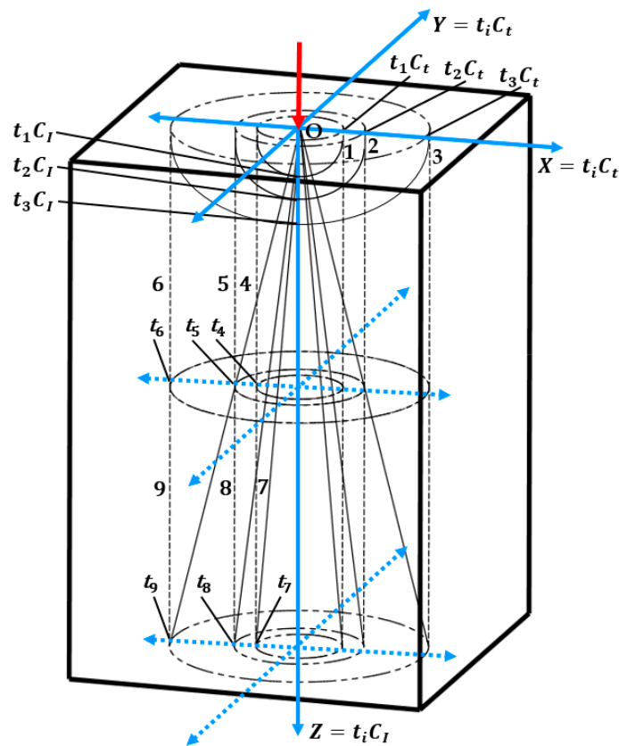
Figure 3. Three-dimensional diagrams of elastic wave propagation.
