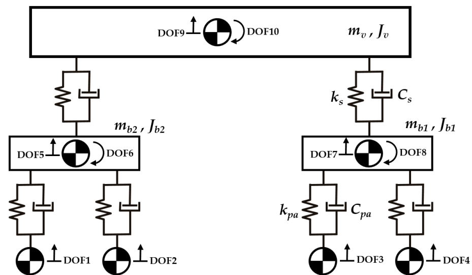
Figure 8. Train half-car numerical model.
