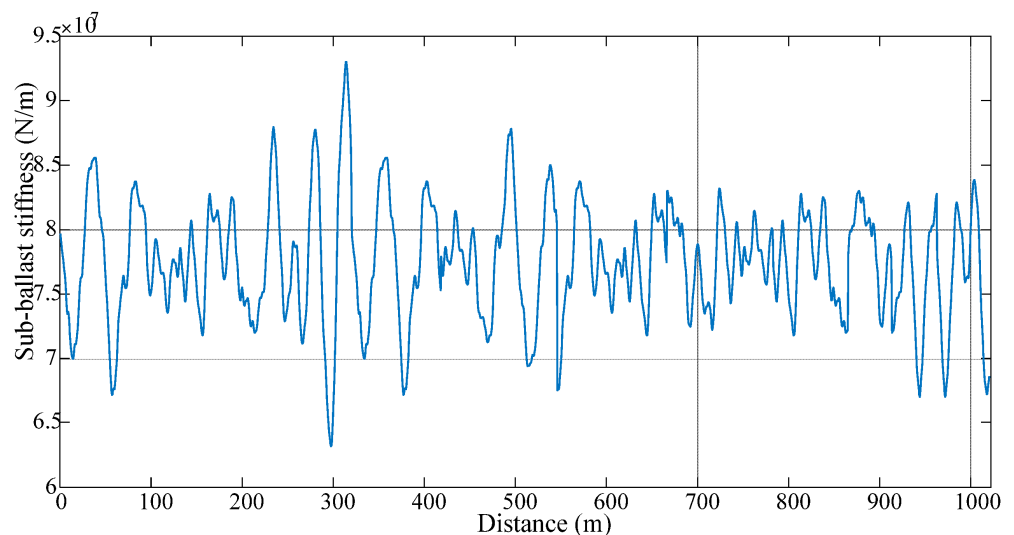
Figure 7. Distribution of the sub-ballast stiffness over distance [49].
