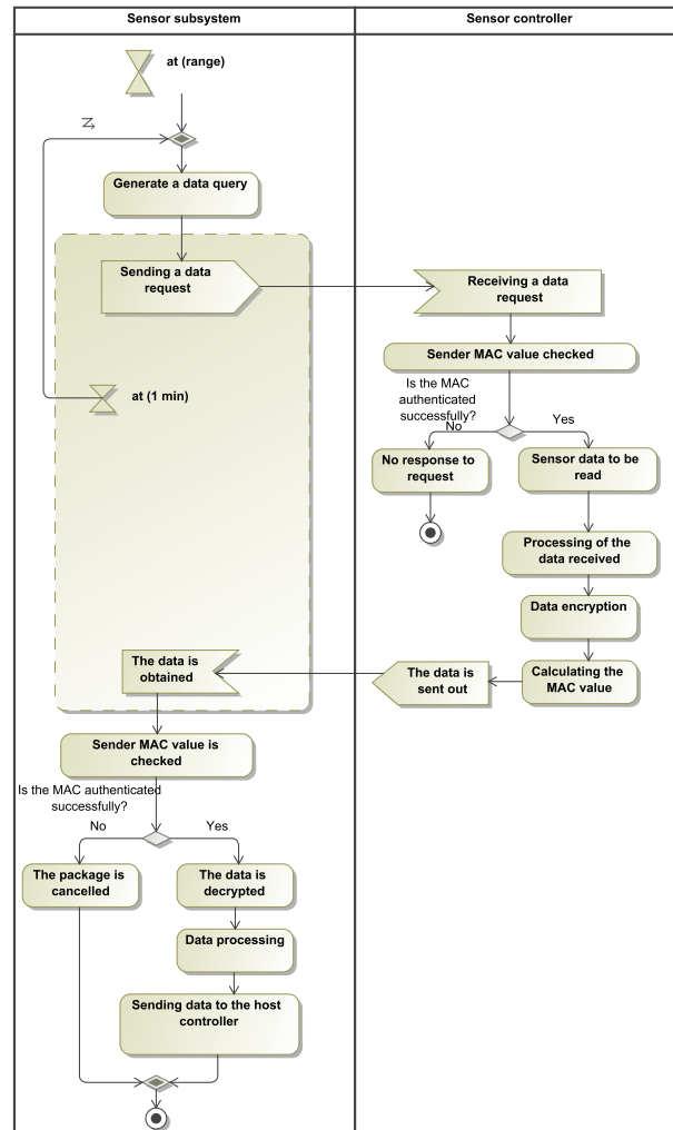
Figure 4. The algorithm for the management of the authentication.
