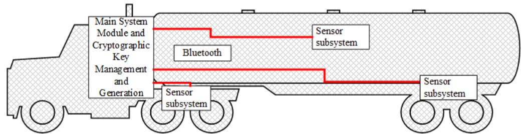
Figure 1. The general concept of the communication security framework for in-vehicle wireless sensor network.
