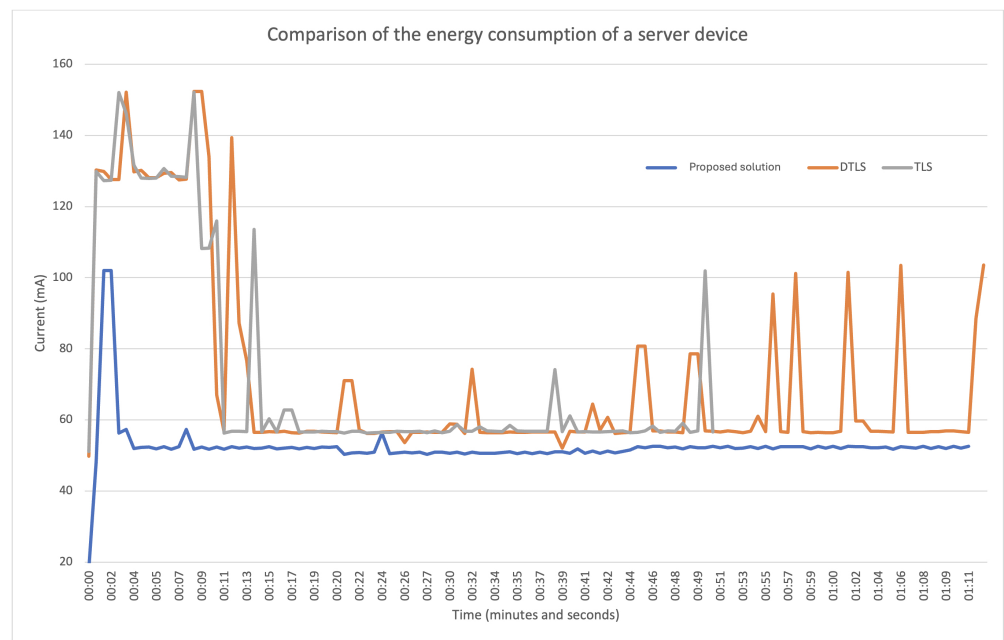
Figure 19. Server device energy comparison chart.
