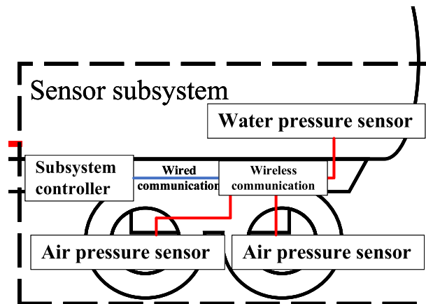
Figure 2. The wireless communication system.
