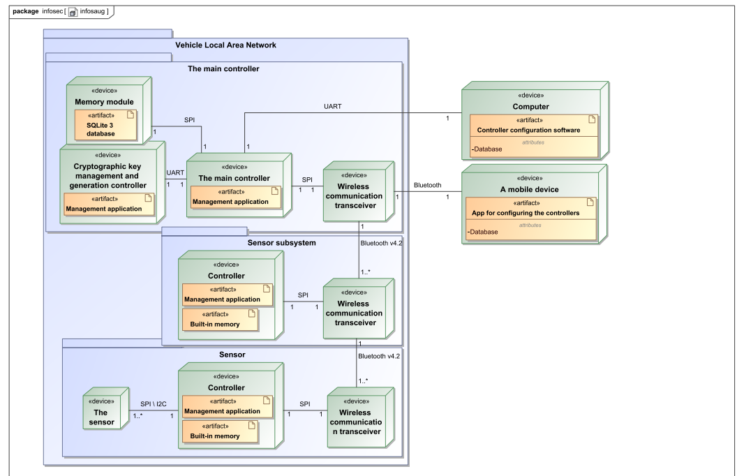
Figure 5. The architecture of the communication between different subsystems.
