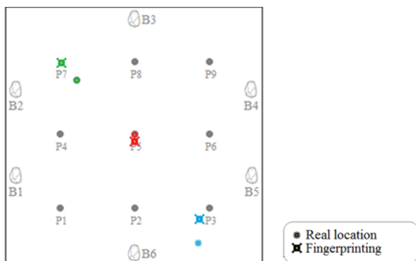
Fig. 3. The visual result of fingerprinting localization algorithm
