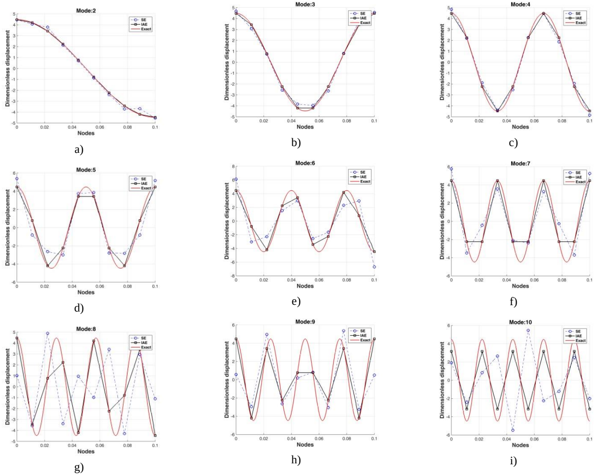
Figure 4. Modified modal shapes of several modes participating in the synthesis of SE60: exact (red smooth line), obtained by direct mapping on the SE (black broken line), modified by optimization for the synthesis of SE60 (dashed line)
