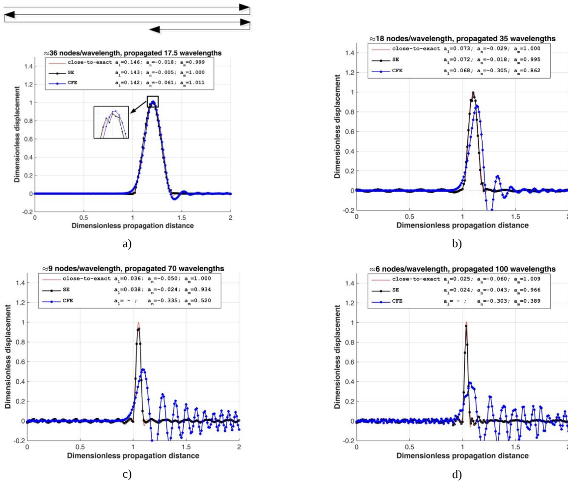
Figure 7. Simulation results after 7 (s): a) \text{delta}T = 0.4 , 36 nodes per wavelength, pulse propagated 17.5 wavelengths; b) \text{delta}T = 0.2 , 18 nodes per wavelength, pulse propagated 35 wavelengths; c) \text{delta}T = 0.1 , 9 nodes per wavelength, pulse propagated 70 wavelengths; d) \text{delta}T = 0.07 , \approx 6 nodes per wavelength, pulse propagated 100 wavelengths
