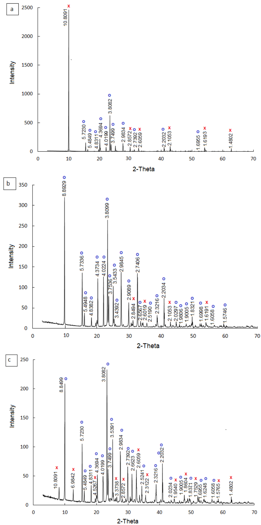
Figure 3. XRD curve of UP produced with a different stoichiometric ratio PWWA:IU, when crystallization time 60 min: (a)—1.5:1.0; (b)—1.0:1.0; (c)—1.0:1.5; x—unidentified, o—urea phosphate.
