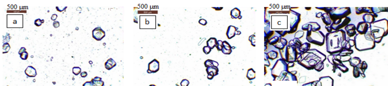
Figure 6. Microscope photographs of UP crystals obtained at a stoichiometric ratio PWPA:IU = 1.0:1.0 and a crystallization time: (a)—at the beginning of crystallization; (b)—after 30 min; (c)—after 60 min.
