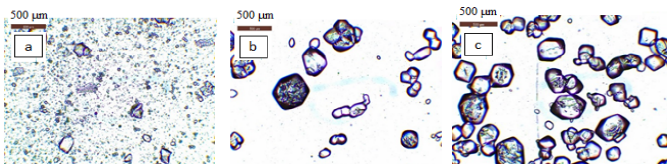
Figure 5. Microscope photographs of UP crystals obtained at a stoichiometric ratio PWPA:IU = 1.5:1.0 and a different crystallization time: (a)—at the beginning of crystallization; (b)—after 30 min; (c)—after 60 min.
