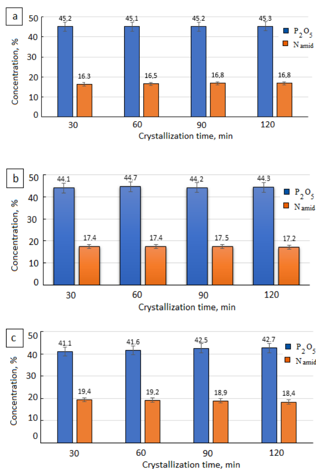
Figure 1. Dependence of the concentration of N amid and P 2 O 5 , on the duration of crystallization when UP is made from PWPA and IU at a stoichiometric ratio: (a)—1.5:1.0; (b)—1.0:1.0; (c)—1.0:1.5.
