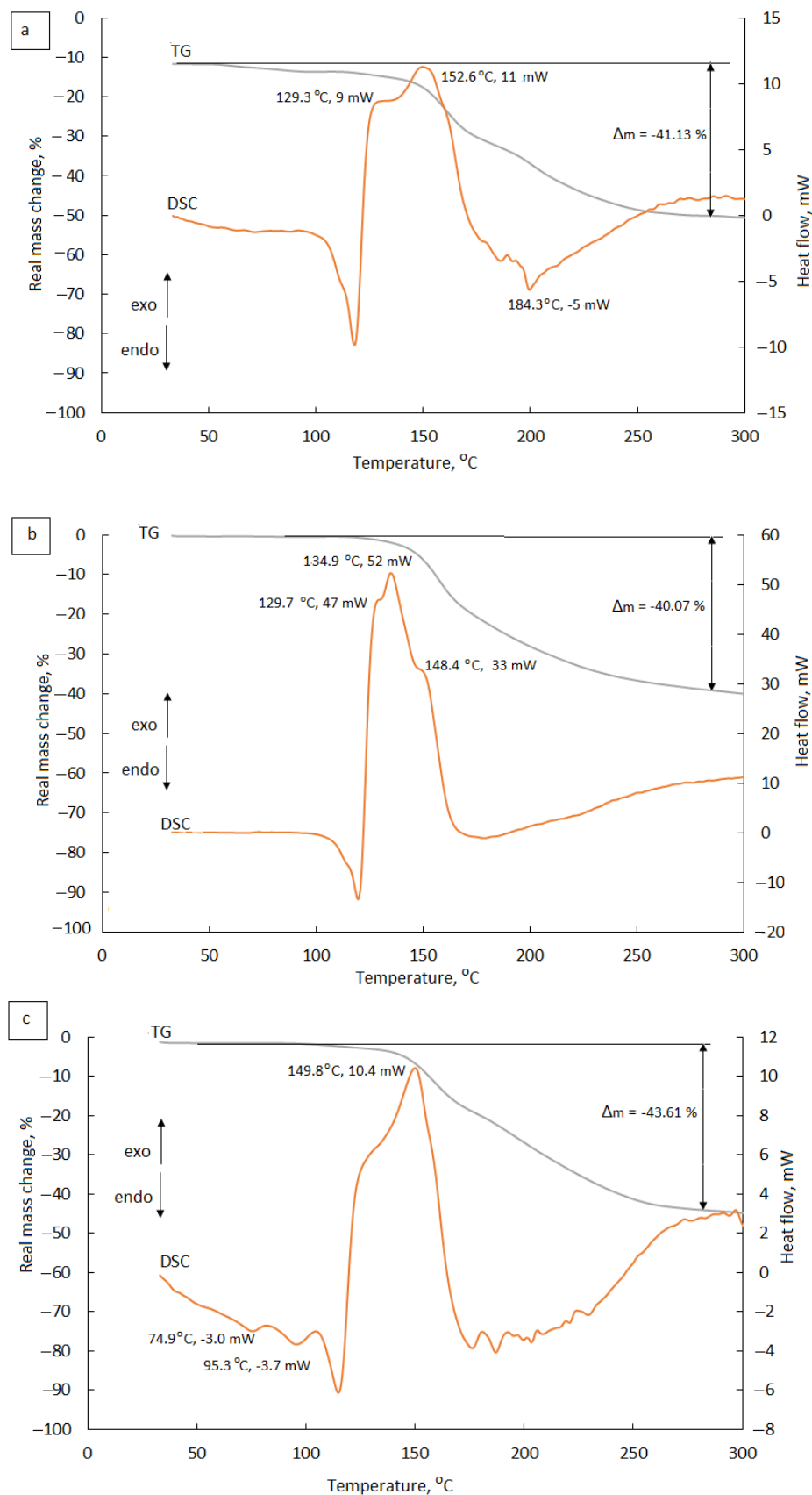
Figure 4. STA curves of the UP produced with a different stoichiometric ratio PWWA:IU, when crystallization time is 60 min: (a)—1.5:1.0; (b)—1.0:1.0; (c)—1.0:1.5.
