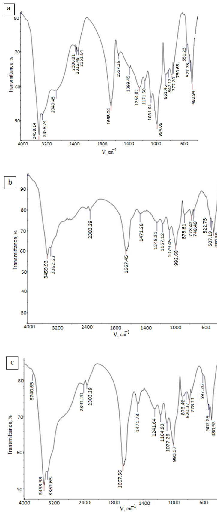
Figure 2. FTIR spectrum of UP produced with a different stoichiometric ratio PWPA:IU, when crystallization time is 60 min: (a)—1.5:1.0; (b)—1.0:1.0; (c)—1.0:1.5.
