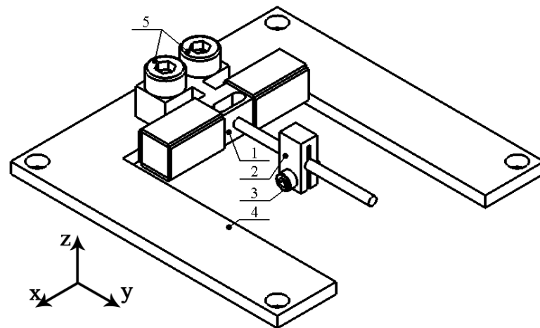
Figure 1. Design of the linear actuator: 1—stator of the actuator; 2—slider; 3—bolt for slider clamping; 4—printed circuit board; and 5—bolts for stator clamping.
