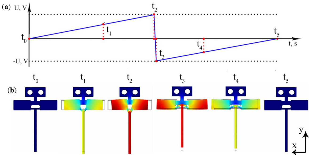
Figure 10. The operation sequence of the actuator: (a) sawtooth excitation signal; (b) sequence of actuator motions.
