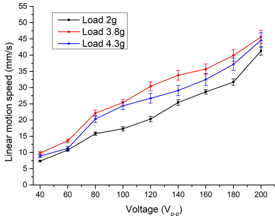
Figure 15. Motion speed characteristics under different loads and excitation signal amplitudes.
