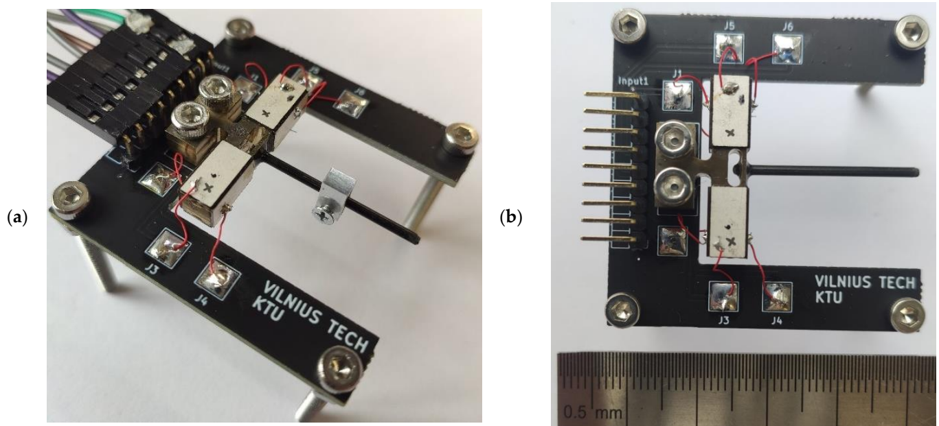
Figure 12. Prototype of the actuator: (a) side view; (b) top view.
