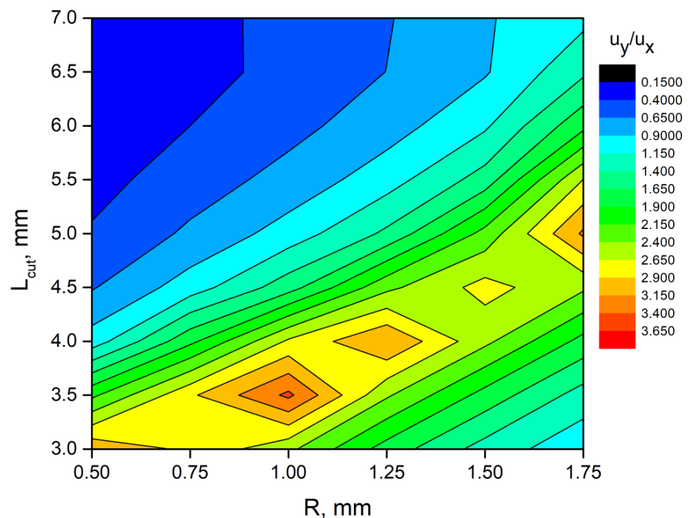
Figure 6. Amplification ratio between output and input displacement amplitudes at different geometrical parameters.
