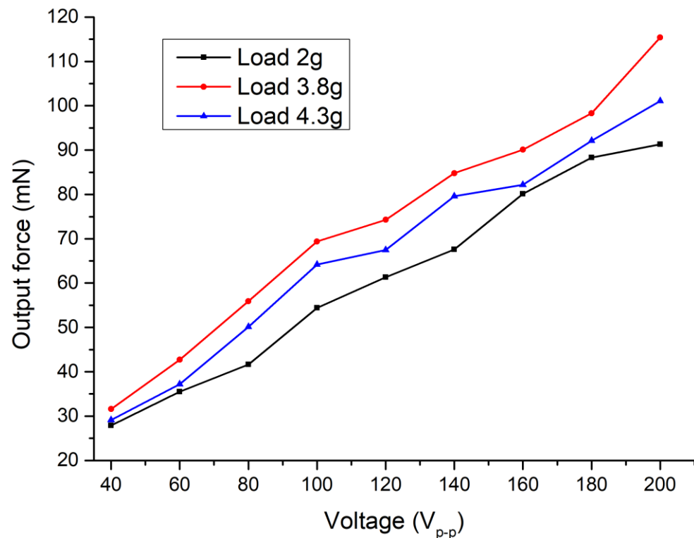
Figure 16. Output force characteristics at different loads and excitation signal amplitudes.
