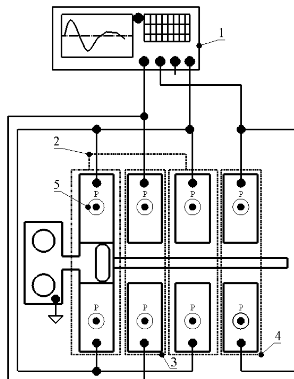
Figure 4. Excitation schematics of actuator; 1—signal generator; 2—group of piezo ceramic plates used to excite longitudinal vibrations; 3—the first group of piezo ceramic used to excite bending vibrations; 4—the second group of piezo ceramic plates used to excite bending vibrations; 5—polarization direction of piezo ceramic plates.
