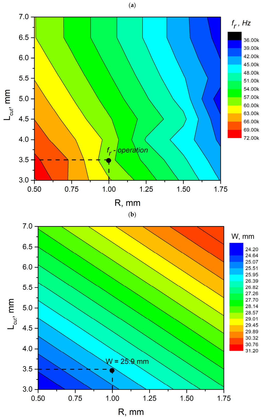
Figure 7. Plots of resonance frequencies and rod lengths are used while different geometrical parameters are used: (a) resonant frequencies of the first longitudinal vibration mode; (b) lengths of square-shaped rod.
