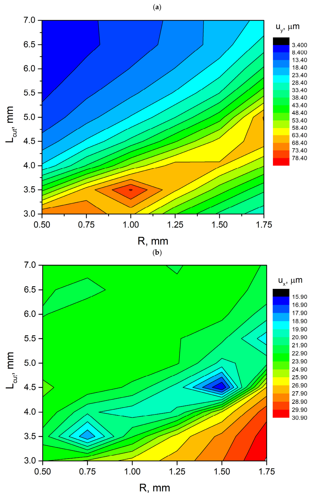
Figure 5. Displacement amplitudes of the actuator in the first longitudinal vibration mode while different geometrical parameters are applied: (a) longitudinal displacement of the guidance rail and (b) longitudinal displacement amplitude of the square-shaped rod.
