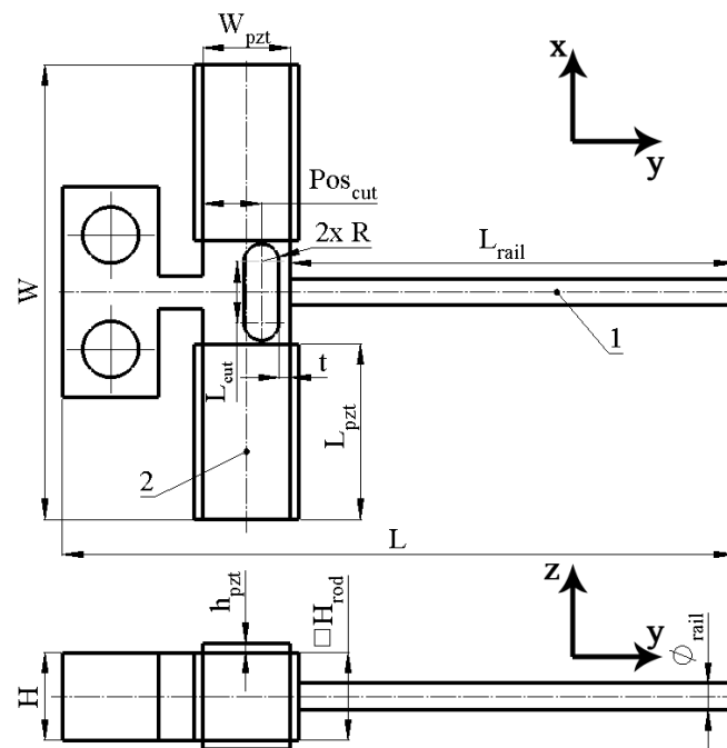
Figure 3. Sketch of the actuator; 1—horizontal axis of symmetry of actuator; 2—longitudinal axis of square rod.
