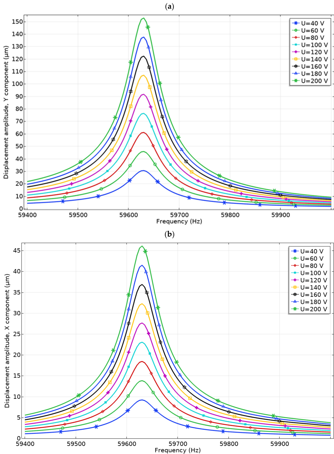
Figure 11. Displacement amplitudes of the actuator; (a) displacements of cylindrical guidance rail in the y direction; (b) displacements of square-shaped rod in the x direction.
