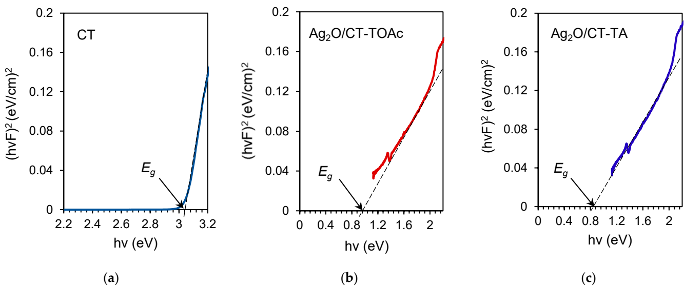
Figure 7. E_g determination from R_d spectra by means of the Kubelka-Munk method.
