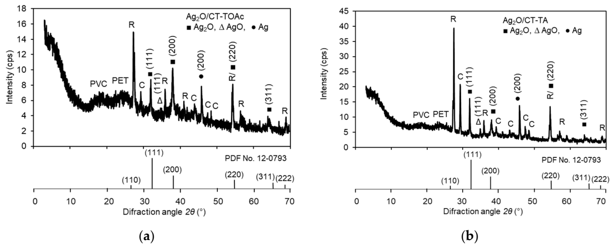
Figure 10. XRD patterns of the \text{Ag}_2\text{O}/\text{CT-TOAc} (a) and \text{Ag}_2\text{O}/\text{CT-TA} (b) composites after cyclic multi-variable aging. Indexes: C—calcite, R—rutile, PET—polyethylene terephthalate, PVC—polyvinylchloride, when ■ is \text{Ag}_2\text{O} , \Delta is \text{AgO} , and • is Ag.
