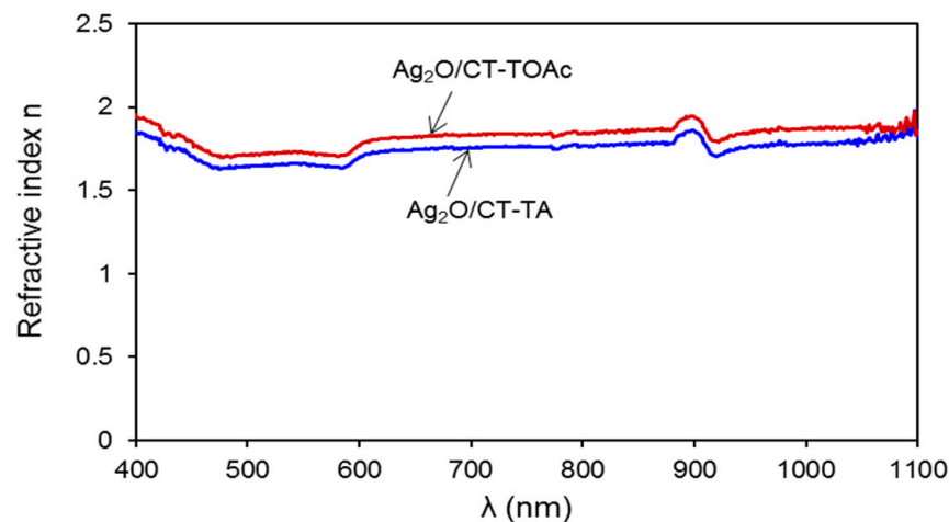
Figure 8. The dependence of refractive indices for Ag 2 O films on the CT surface in terms of wavelength.
