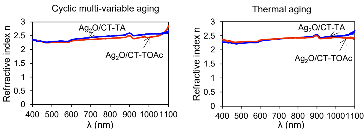
Figure 13. The dependence of refractive indices for \text{Ag}_2\text{O} films on the CT surface after cyclic multi-variable and thermal aging in terms of wavelength.
