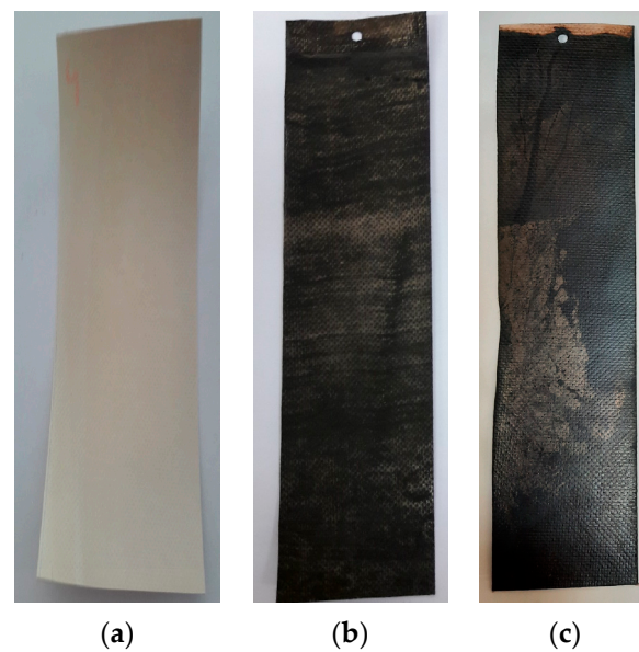
Figure 4. Samples used for the tests: (a) roughened CT side; (b) \text{Ag}_2\text{O}/\text{CT-TA} ; and (c) \text{Ag}_2\text{O}/\text{CT-TOAc} .
