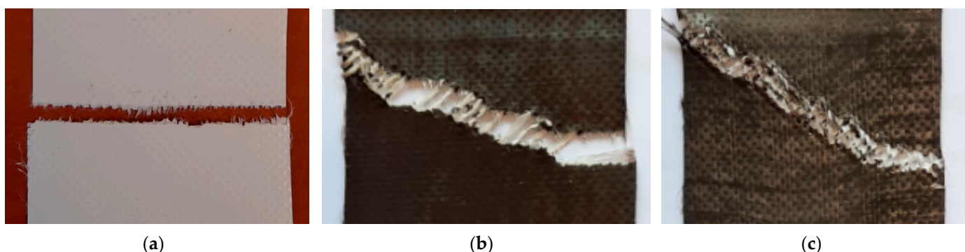
Figure 16. Failure modes for CT (a), Ag 2 O/CT-TOAc (b), and Ag 2 O/CT-TA (c) samples in tensile tests.
