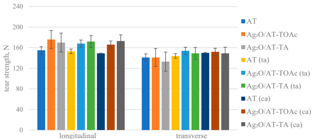
Figure 14. Tear strength results of initial and thermo-chemically treated CT before and after thermal (ta) and cyclic multi-variable (ca) aging.
