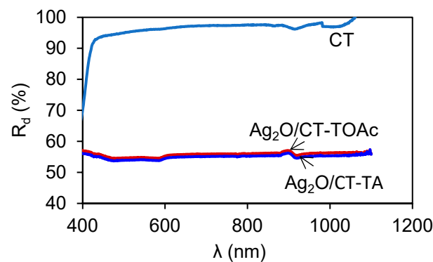
Figure 6. Measured R_d spectra of CT and Ag_2O films deposited on different pretreated CT.
