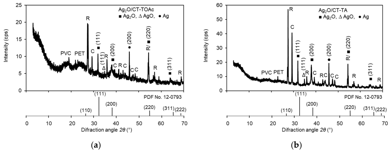
Figure 9. XRD patterns of the \text{Ag}_2\text{O}/\text{CT-TOAc} (a) and \text{Ag}_2\text{O}/\text{CT-TA} (b) composites after thermal aging. Indexes: C—calcite, R—rutile, PET—polyethylene terephthalate, PVC—polyvinylchloride, when ■ is \text{Ag}_2\text{O} , \Delta is \text{AgO} , and • is Ag.
