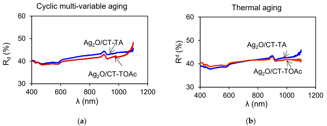
Figure 11. Measured R_d spectra of the Ag_2O films deposited on different pre-treated CT after cyclic multi-variable and thermal aging.
