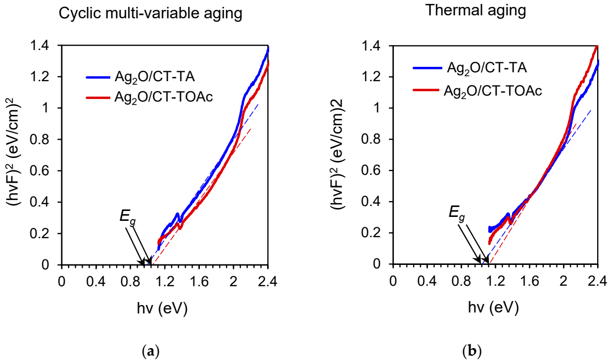
Figure 12. E_g determination from R_d spectra by means of the Kubelka-Munk method after cyclic multi-variable and thermal aging.
