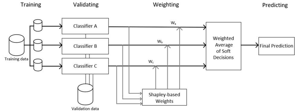
Figure 2. Overview of the proposed ensemble weight calculation strategy.
