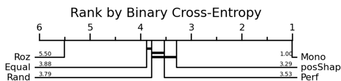
Figure 20. Ranking of heterogenous ensembles: using BNG-credit_a dataset and R implementation.
