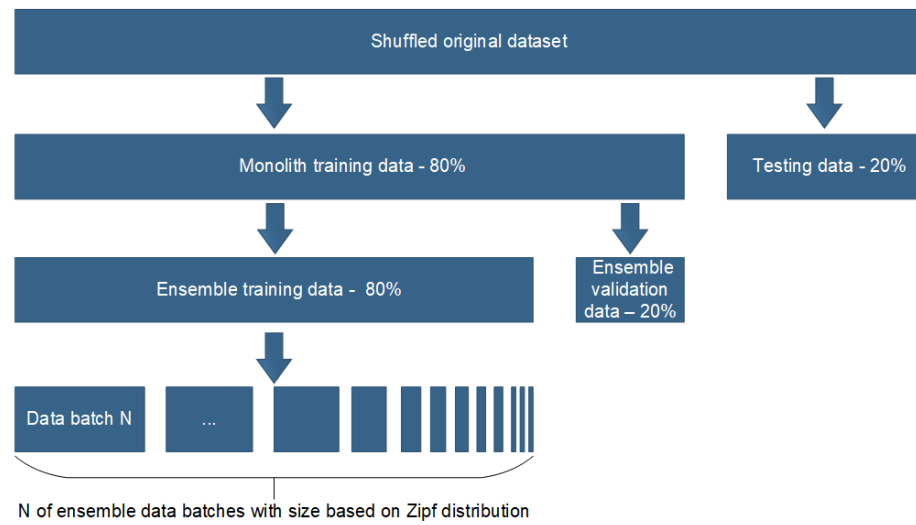
Figure 4. Double hold-out validation scheme with Zipf-derived data splitting for training ensemble members.
