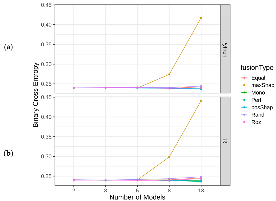
Figure 9. Detection error by BCE for various homogenous ensemble sizes: logistic regression in Python (a) and R (b) using Bank Marketing dataset.
