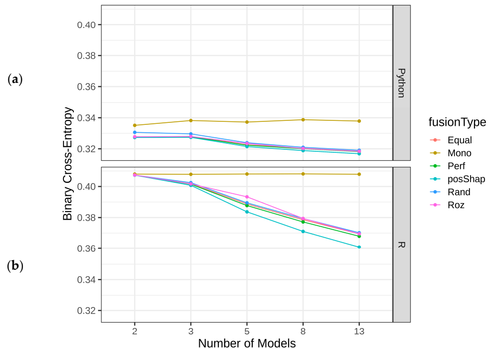
Figure 7. Detection error by BCE for various homogenous ensemble sizes: decision tree in Python (a) and R (b) using BNG_credit-a dataset.
