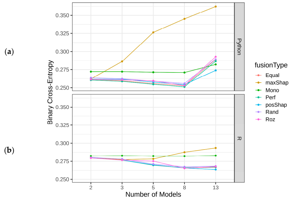
Figure 11. Detection error by BCE for various homogenous ensemble sizes: decision tree in Python (a) and R (b) using Bank Marketing dataset.
