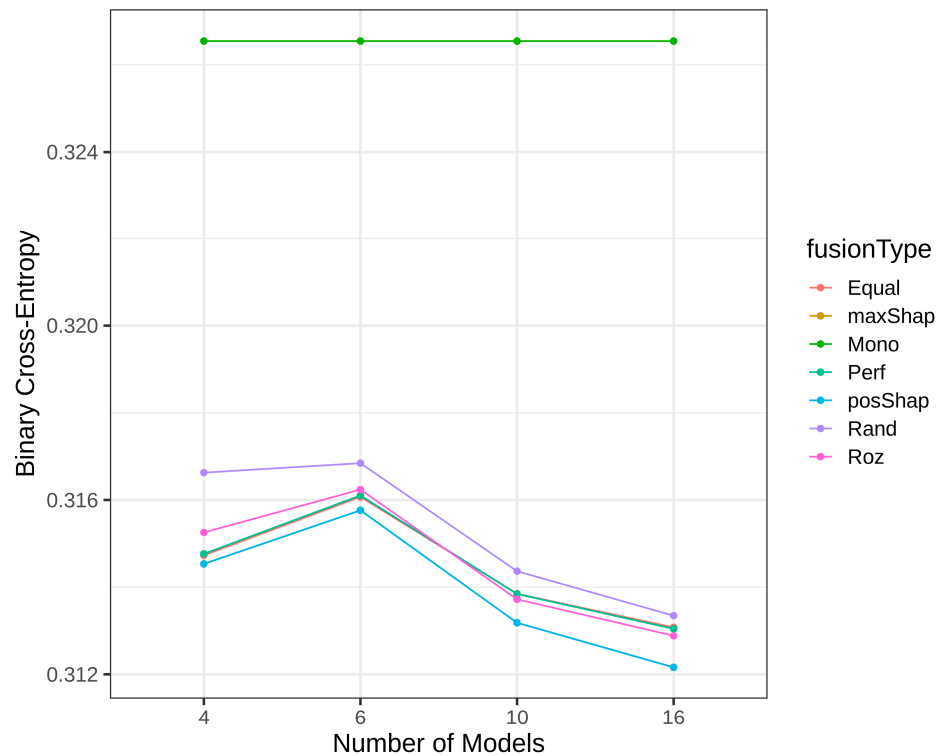
Figure 15. Detection error by BCE for various heterogenous ensemble sizes using Python models and BNG-credit_a dataset.
