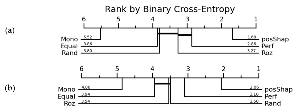
Figure 8. Ranking of homogenous ensembles: decision tree in Python (a) and R (b) using BNG_credit-a dataset.
