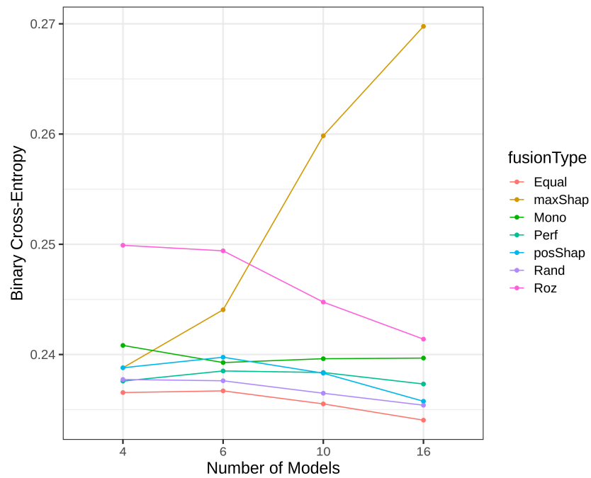
Figure 17. Detection error by BCE for various heterogenous ensemble sizes using R models and Bank Marketing dataset.
