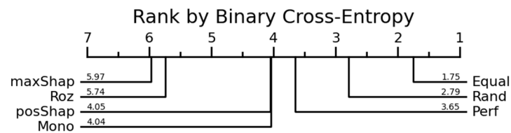
Figure 18. Ranking of heterogenous ensembles: using Bank Marketing dataset and R implementation.
