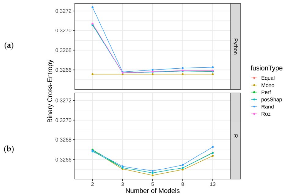
Figure 5. Detection error by BCE for various homogenous ensemble sizes: logistic regression in Python (a) and R (b) using BNG_credit-a dataset.
