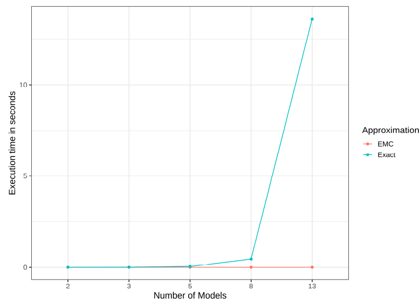
Figure 21. Runtime comparison of Shapley-based weighting strategies used in experiments. Note: exact was used in the maxShap or posShap strategies and EMC was used in Roz strategy [19].
