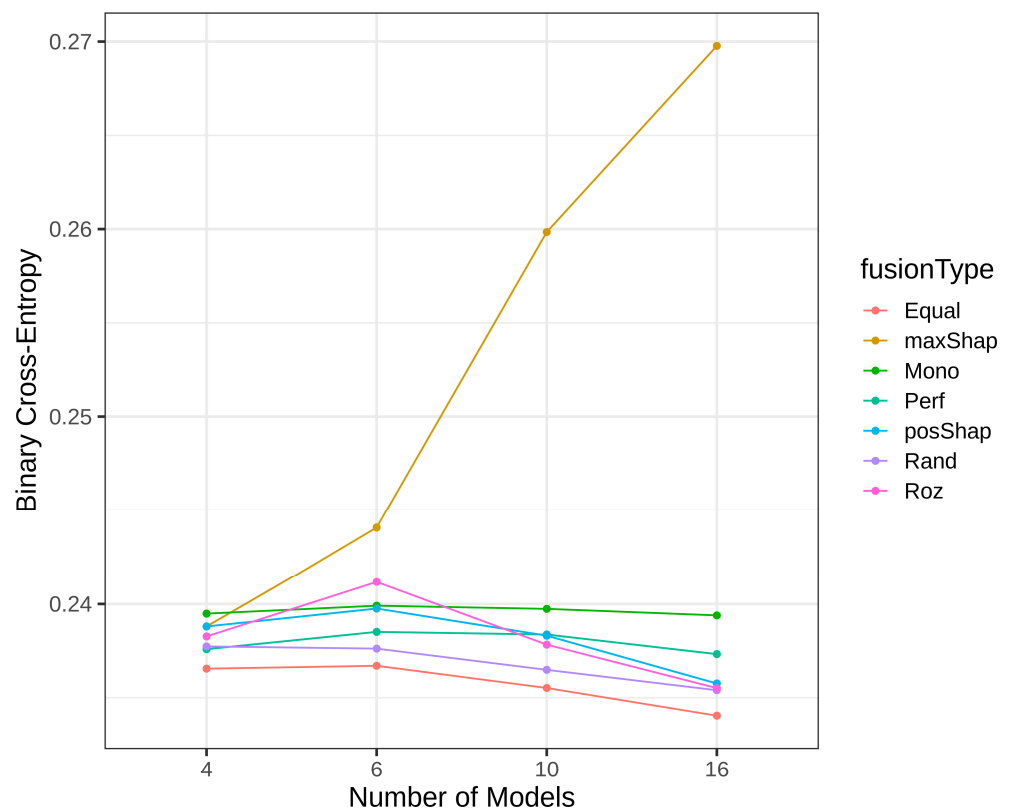
Figure 13. Detection error by BCE for various heterogenous ensemble sizes using Python models and Bank Marketing dataset.
