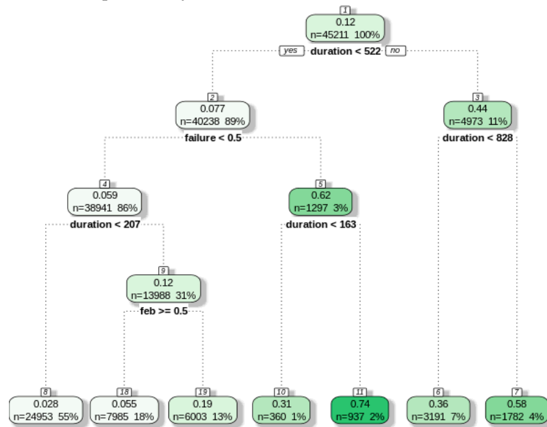
Figure 3. Decision tree visualization for Bank Marketing dataset, where the darker the color of the node the more target class cases (clients subscribed to the service) of the training data exist there.
