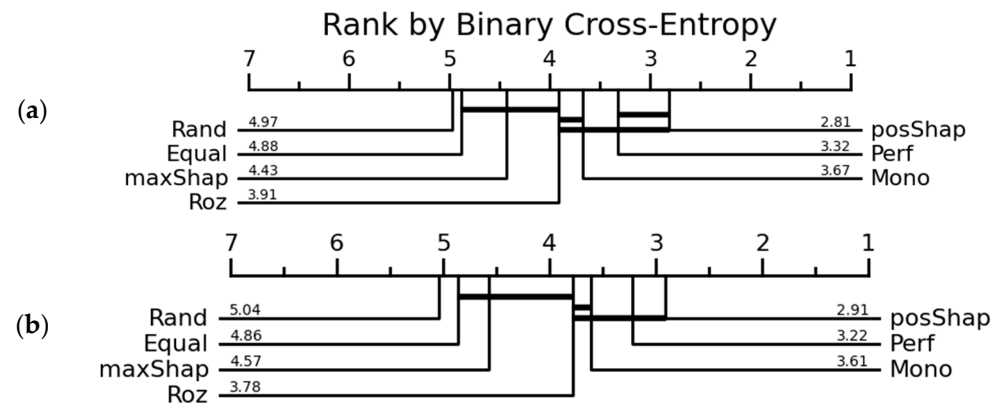
Figure 10. Ranking of homogenous ensembles: logistic regression in Python (a) and R (b) using Bank Marketing dataset.
