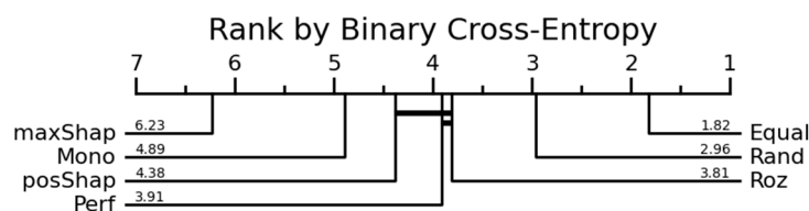
Figure 14. Ranking of heterogenous ensembles: using Bank Marketing dataset and Python implementation.
