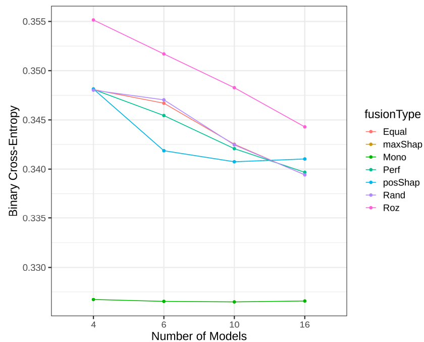
Figure 19. Detection error by BCE for various heterogenous ensemble sizes using R models and BNG-credit_a dataset.
