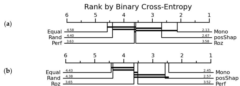
Figure 6. Ranking of homogenous ensembles: logistic regression in Python (a) and R (b) using BNG_credit-a dataset.
