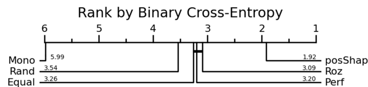
Figure 16. Ranking of heterogenous ensembles: using BNG-credit_a dataset and Python implementation.
