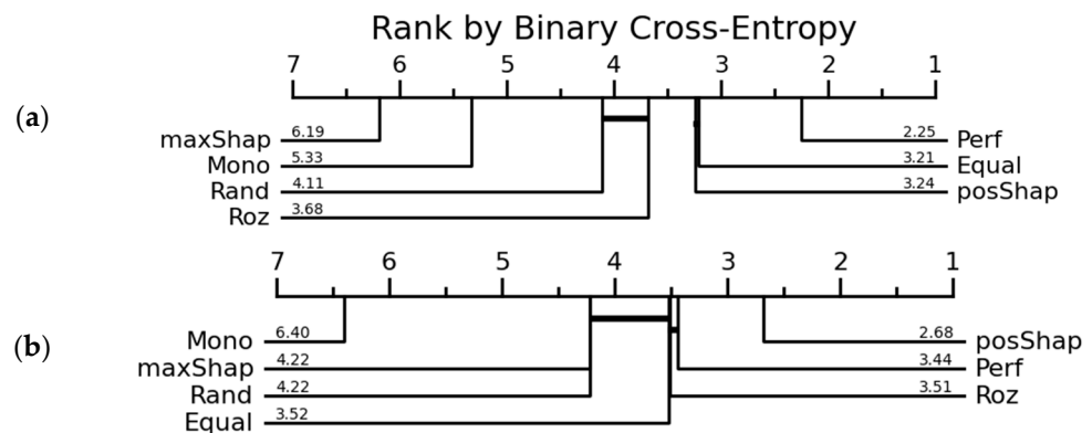
Figure 12. Ranking of homogenous ensembles: decision tree in Python (a) and R (b) using Bank Marketing dataset.
