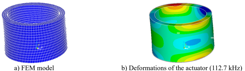
Fig. 2. Numerical modelling of the cylindrical actuator
