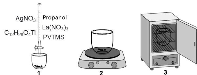
Figure 2. Synthesis route for nanocomposites.
