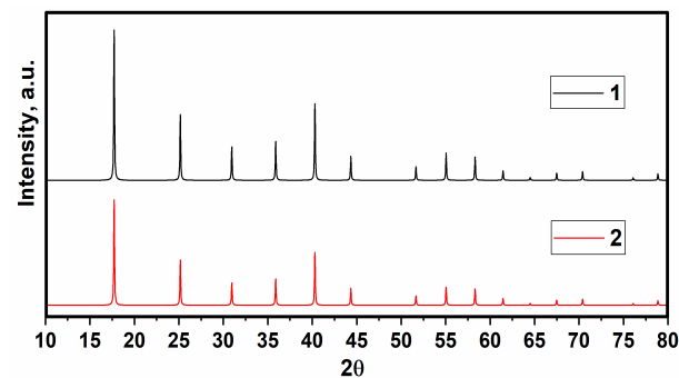
Figure 3. X-ray diffraction of nanocomposites 1 and 2.
