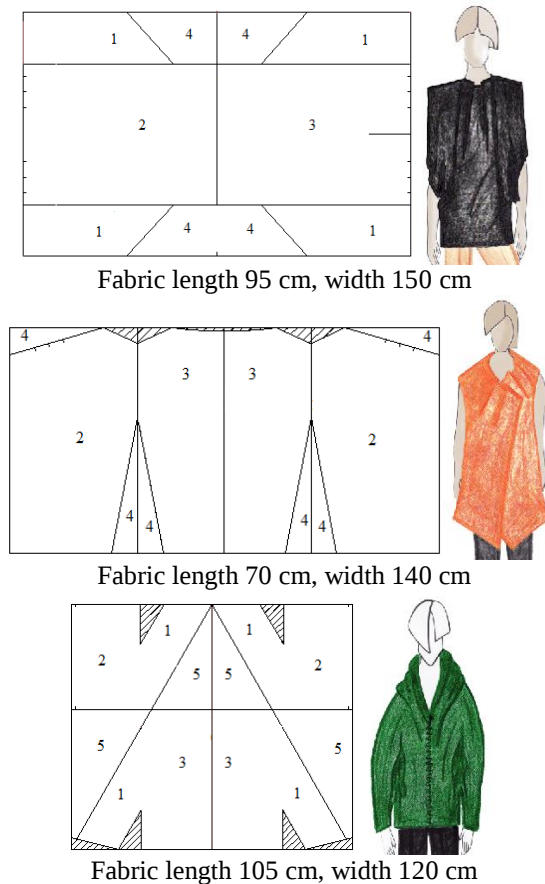
Figure 2. Constructions of 3 collection models created following zero waste principles. Marking: 1 – sleeve, 2 – front, 3 – back, 4 – hem, 5 – hood.
