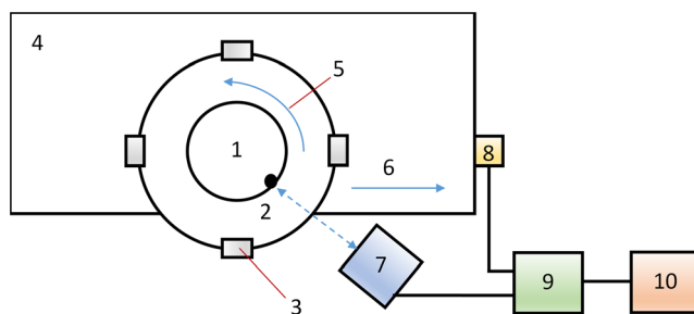
Fig. 18 Structural scheme of the vibrodiagnostic stand for mill technical state evaluation: 1 mill axis; 2 mark of tachometer signal; 3 mill teeth; 4 work piece; 5 direction of mill rotation; 6 feed direction of the work piece; 7 shaper of tachometer signal; 8 accelerometer; 9 oscilloscope; 10 PC with vibrodiagnostic analysis software
