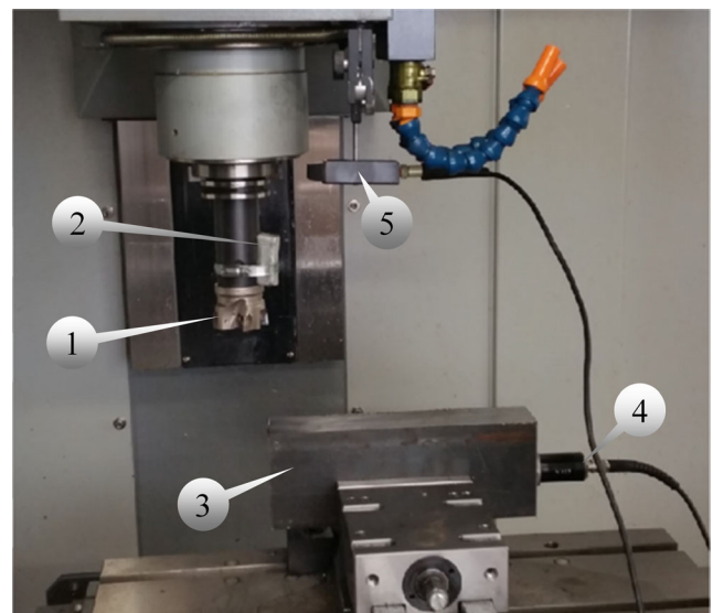
Fig. 19 General view of the set-up of the technical state evaluation sensors of the mill: 1 mill; 2 Wi-Fi vibrational level sensor; 3 work piece; 4 accelerometer BK-310A; 5 transmitter of tachometer signal
