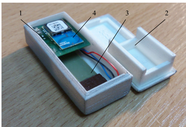
Fig. 5 General view of the electrical energy harvester (length × width × depth = 44 × 20 × 18 mm, mass 13.8 g): 1 case; 2 cover; 3 piezoelectric cantilever of type CMBP05 (Noliac A/S, Denmark), 4 controller with wireless transmitter
