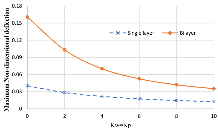
Figure 12. The variation of the nondimensional maximum deflection for the circular nanoplate for single-layer and bilayer nanoplates.
