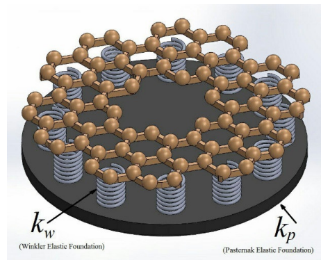
Figure 1. The graphene annular plate on elastic foundations.
