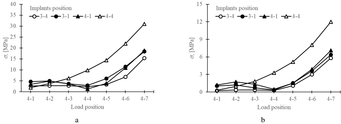
Fig. 2 Dependence of stress on the position of occlusion load, when diameter of implants is 3.5 mm (a) and 4.5 mm (b) and implants position is at 34-31-41-44
