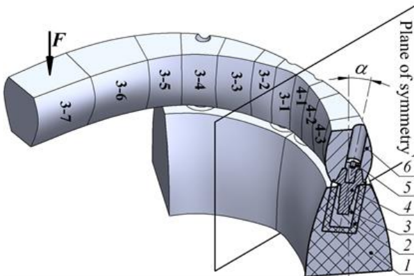
Fig. 1 The design of modelled structure
