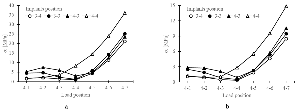
Fig. 4 Dependence of stress on the position of occlusion load, when diameter of implants is 3.5 mm (a) and 4.5 mm (b) and implants position is at 34-33-43-44
