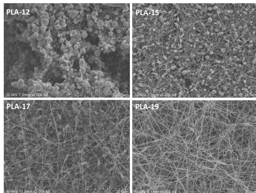
Figure 3. SEM images of pure PLA nanofibers with concentrations of 12, 15, 17, and 19% (scale—20 \mu\text{m} ).
