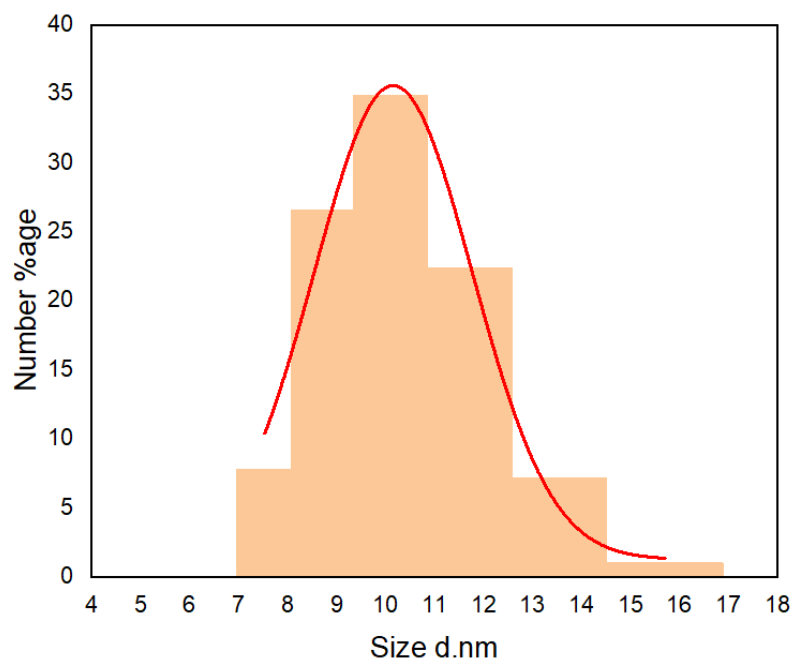
Figure 6. Size distribution of prepared CNDs measured by DLS.
