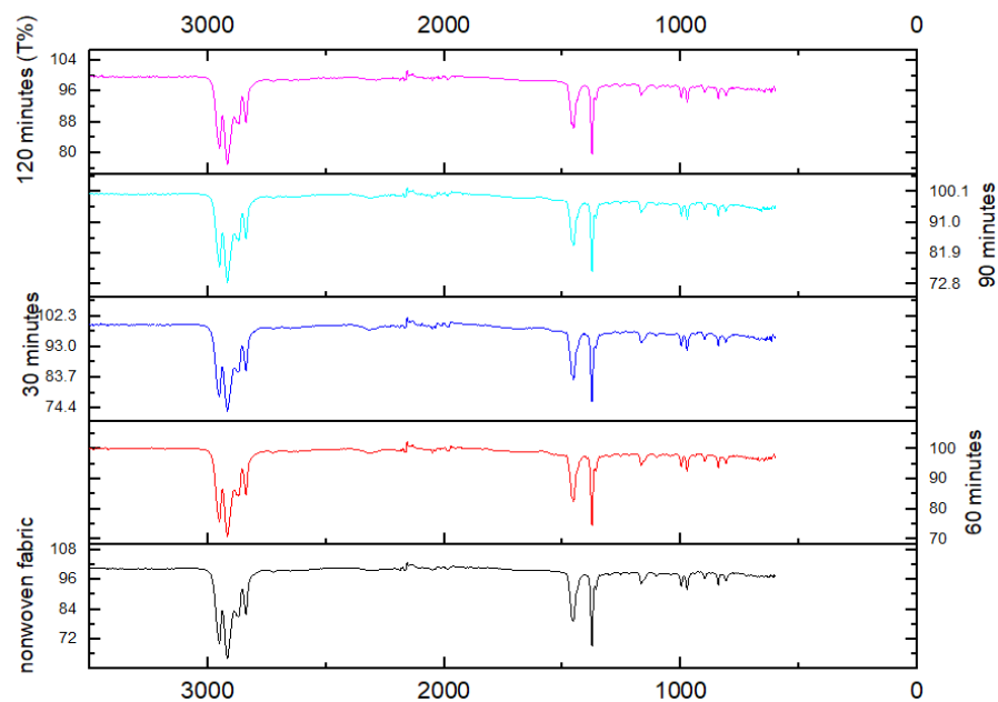
Figure 10. FTIR spectra of PLA-19/C4 samples at different electrospinning times.
