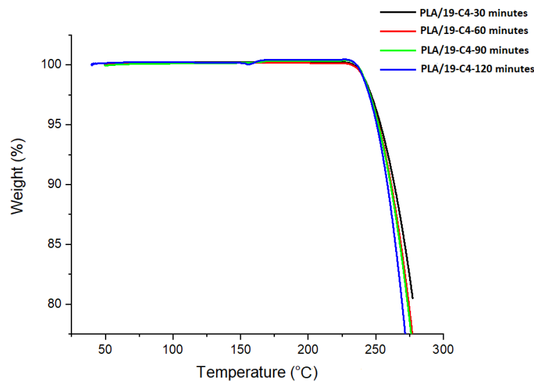
Figure 11. TGA analysis of PLA-19/C4 electrospun fibers.
