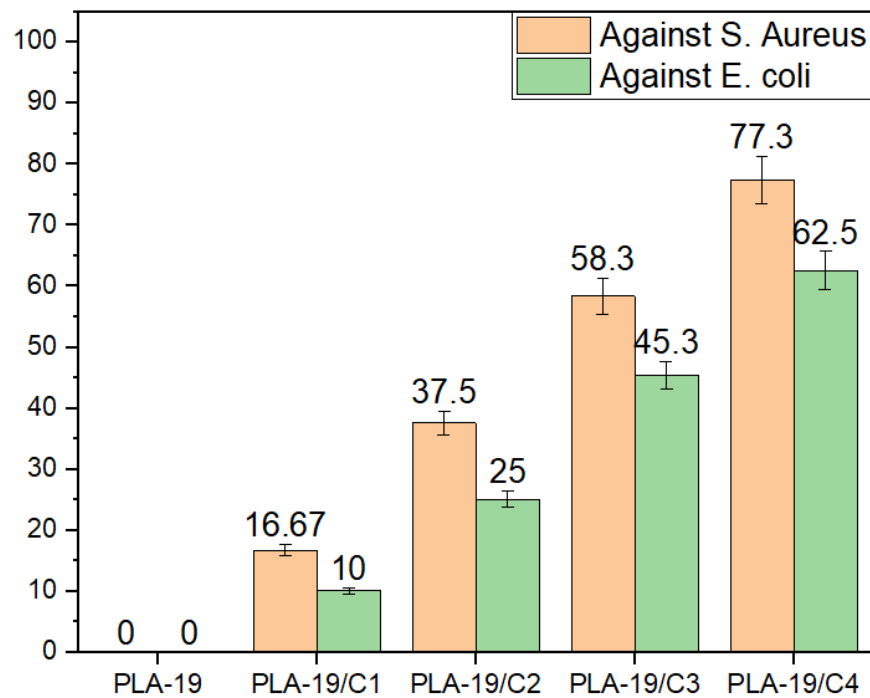
Figure 7. Antimicrobial activity of PLA-19/C1, PLA-19/C2, PLA-19/C3 and PLA-19/C4 against S. aureus and E. coli .
