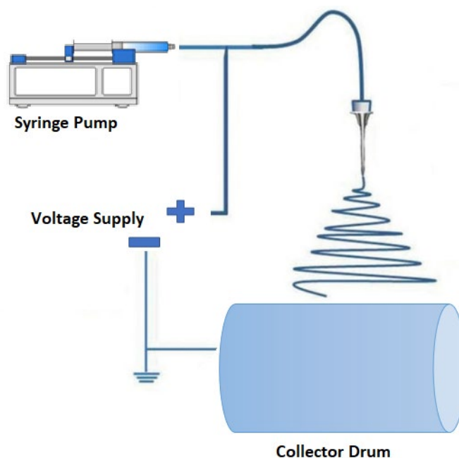
Figure 2. Electrospinning process for PLA nanofibers.
