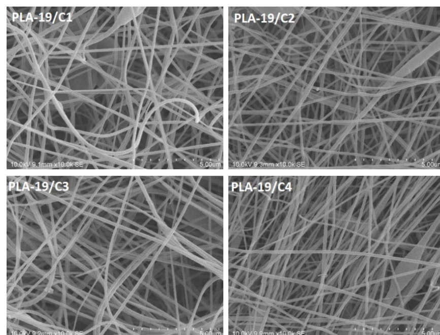
Figure 5. SEM images of 19% PLA nanofibers with variations in CNDs of 1, 2, 3, and 4% (scale—5 μm).
