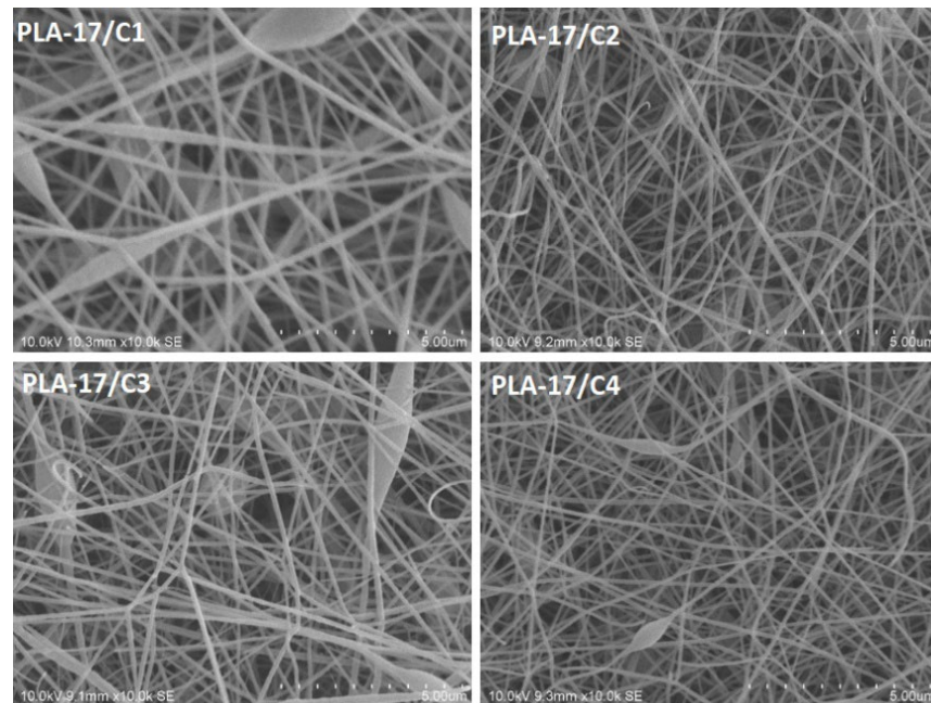
Figure 4. SEM images of 17% PLA nanofibers with variations in the CNDs of 1, 2, 3, and 4% (scale—5 μm).
