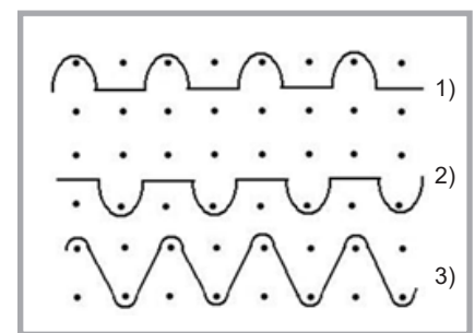
Figure 1. Knitting pattern of materials tested; 1) outer layer - pattern course E3, 2) inner layer - pattern course E2, 3) middle layer - pattern course E1.
