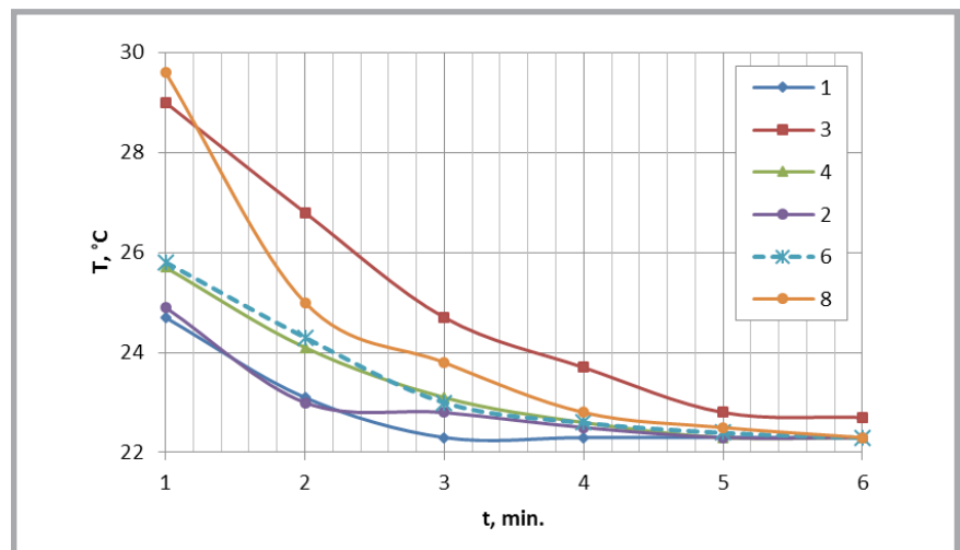
Figure 2. Influence of different methods of bio-ceramic application on textiles' heat release.
