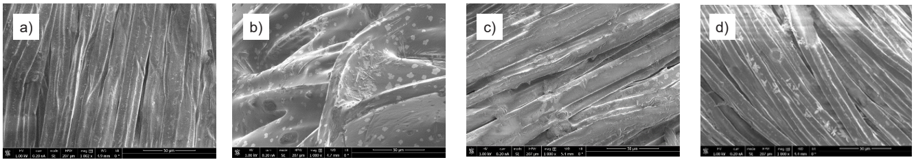
Figure 3. SEM micrographs (original magnification: 1000×) of knitted fabric samples: 1 (a), 3 (b), 6 (c) and 8 (d).
