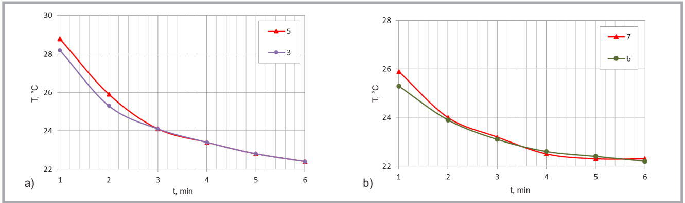
Figure 4. Plasma-treatment influence on textiles' heat release after applying the bio-ceramicscreen-printing (a) and impregnation (b) methods.
