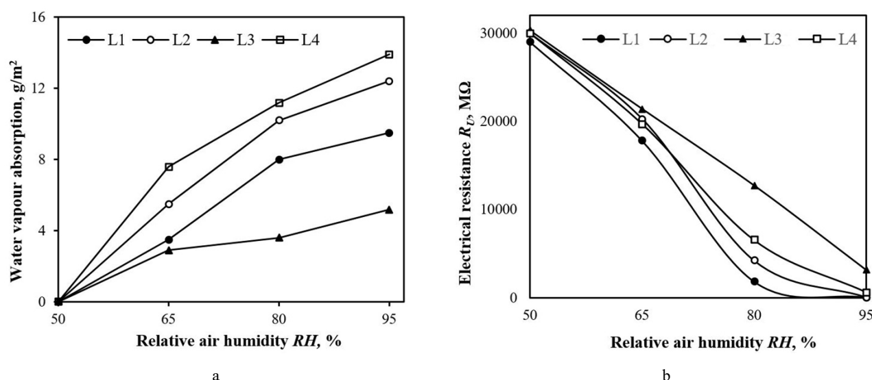
Fig. 2. Dependence of the textile laminates upon the relative humidity: a – water vapour absorption; b – electrical resistance
