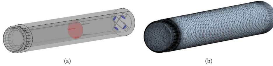
FIGURE 9: Linear motion hydraulic cylinder type MR resistive exercise device for lever-type rowing machine: (a) computational domain geometrical model with boundary conditions; (b) finite element mesh (952.000 volume elements).
