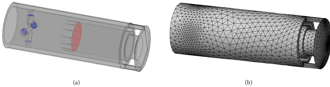
FIGURE 7: Models of MR fluid damper: (a) computational domain with boundary conditions indicated; (b) finite element mesh of computational domain ( \sim 390.000 volume elements).
