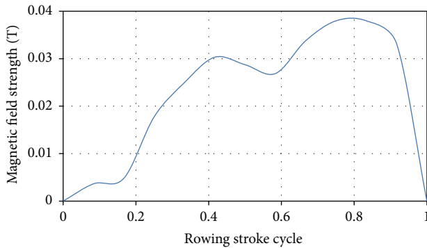
FIGURE 14: Law of variation of magnetic field strength giving the pattern of resistance force corresponding to rowing of the real boat.
