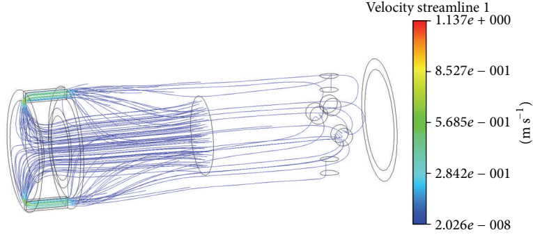
FIGURE 10: Trajectories and velocities of the magnetorheological fluid flow in MR damper in the case of flow input velocity corresponding to 0.0075 m/s piston speed and 25 mT magnetic field.
