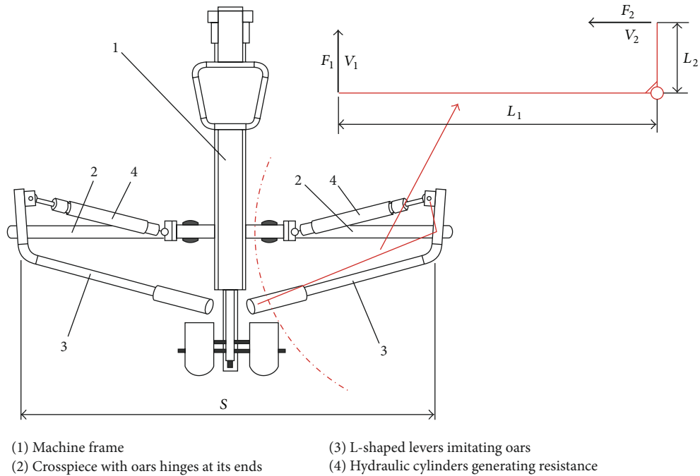
FIGURE 1: Structure of lever-type rowing machine and kinematical scheme of resistance system: S : spread (scull), L_1 and L_2 : lengths of L-shaped levers imitating oar handles ( S = 1.58 m, L_1 = 0.74 m, and L_2 = 0.135 m), F_1 : force on oar handle, and F_2 : resistance force generated by hydraulic cylinder.
