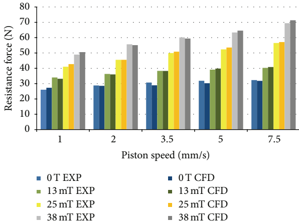
FIGURE 11: Comparison of experimentally determined (EXP) and calculated (CFD) resistance forces generated by a MR damper at different speeds of the piston and different magnetic field strength (0 T; 13 mT; 25 mT; and 38 mT magnetic field).
