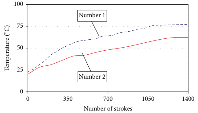
FIGURE 4: Dependencies of the temperature of hydraulic cylinder numbers 1 and 2 on the number of exercise cycles (exercising rate: 50 strokes/min).
