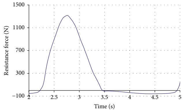
FIGURE 3: The law of change of resistance force generated by hydraulic cylinder type load generating unit of HAMMER Cobra rowing machine during a single stroke cycle (exercising rate 24 strokes/min, resistance level: 5).
