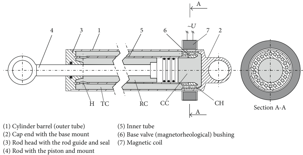
FIGURE 8: Scheme of MR resistive exercise device for rowing machine: CC: compression chamber; RC: rebound chamber; CH: circular channels in the bushing of magnetorheological base valve; TC: tubular chamber; H: radial holes connecting tubular and rebound chambers.
