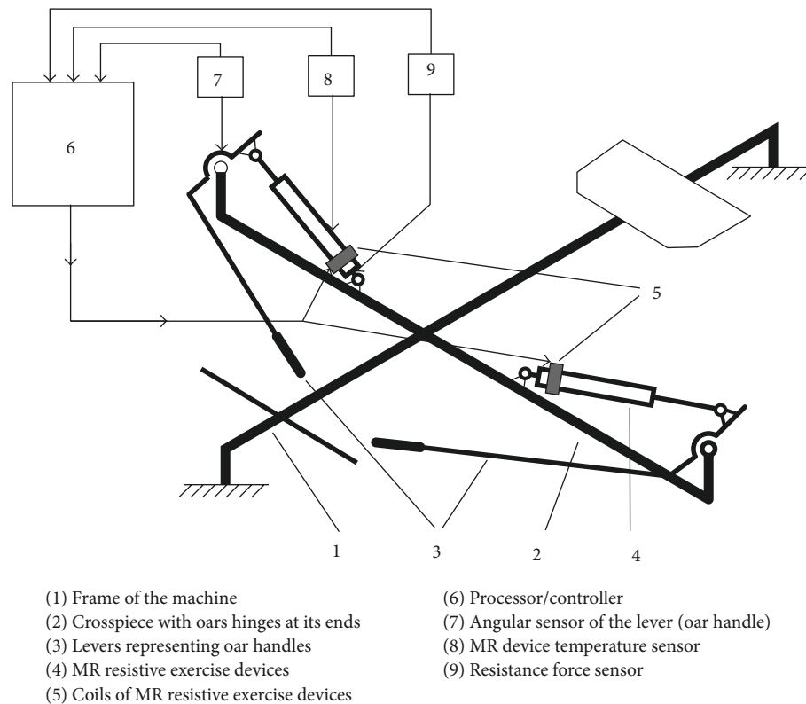
FIGURE 15: Scheme of lever-type rowing machine with the programmable control system of MR resistive exercise device.
