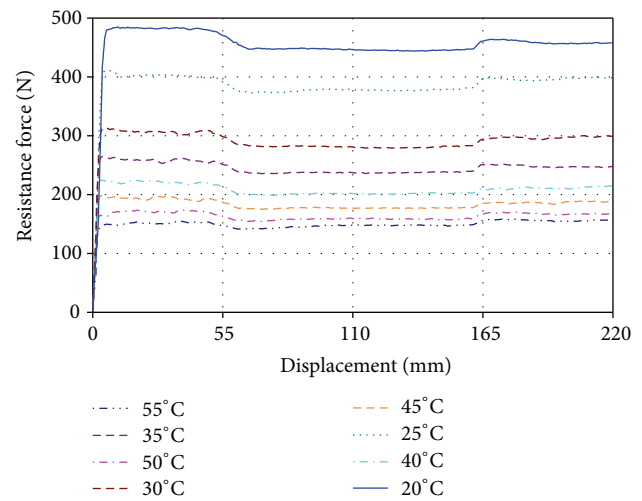
FIGURE 5: Dependencies of the resistance force generated by hydraulic cylinder number 2 on its body temperature (speed of rod/piston extraction: 0.015 m/s).
