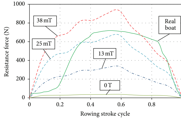
FIGURE 13: The patterns of resistance force on the oar handle when rowing a real boat [20] and when exercising on a rowing machine with MR loading device (at strength of the magnetic field (0 T, 13 mT, 25 mT, and 38 mT)).
