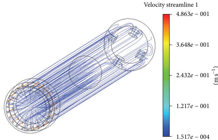
FIGURE 12: Trajectories and velocities of magnetorheological fluid flow in MR resistive exercise device for rowing machine (number of the channels in the base valve bushing for fluid passage between the chambers: 25; diameter: 0.8 mm).
