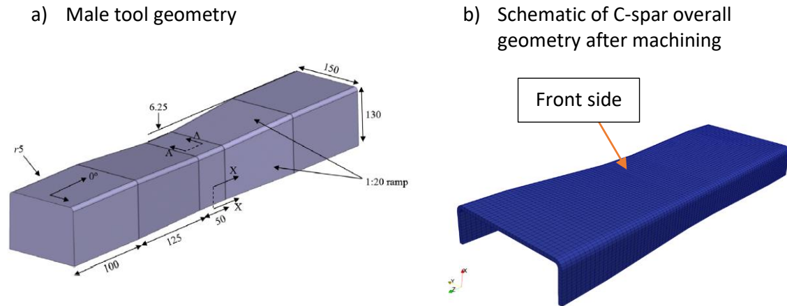
Figure 3: C-Spar Specimen Dimensions from [4]
