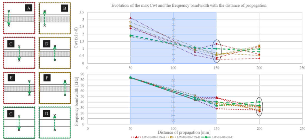
Figure 6: Signals compared for the stiffened delaminated zone analysis.
