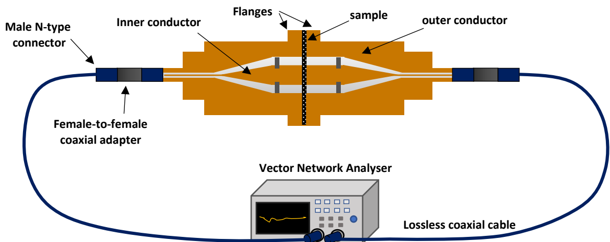
Figure 3. Coaxial transmission line method for measuring shielding effectiveness
