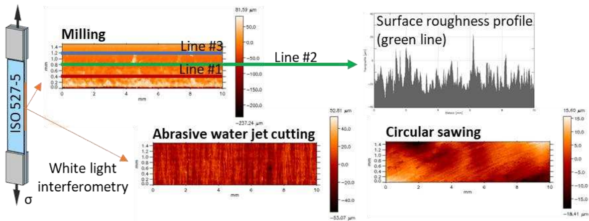
Figure 2. White light interferometry on transverse tensile specimens (ISO 527-5 [21]), 3D roughness analysis and derivation of path profile on section planes
