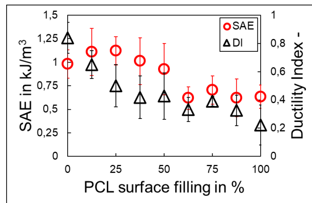
Figure 3. Ductility results at compression after impact test at different surface filling content
