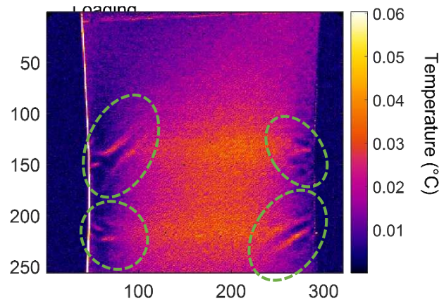
Figure 6: Typical \Delta T image obtained from the web of the C-spar gauge section as seen from the front. Subsurface wrinkles highlighted in green.
