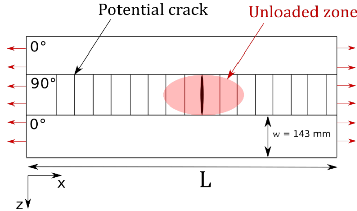
Figure 2. Geometry of the multi-cracked cell associated to a [0/90/0] laminate
