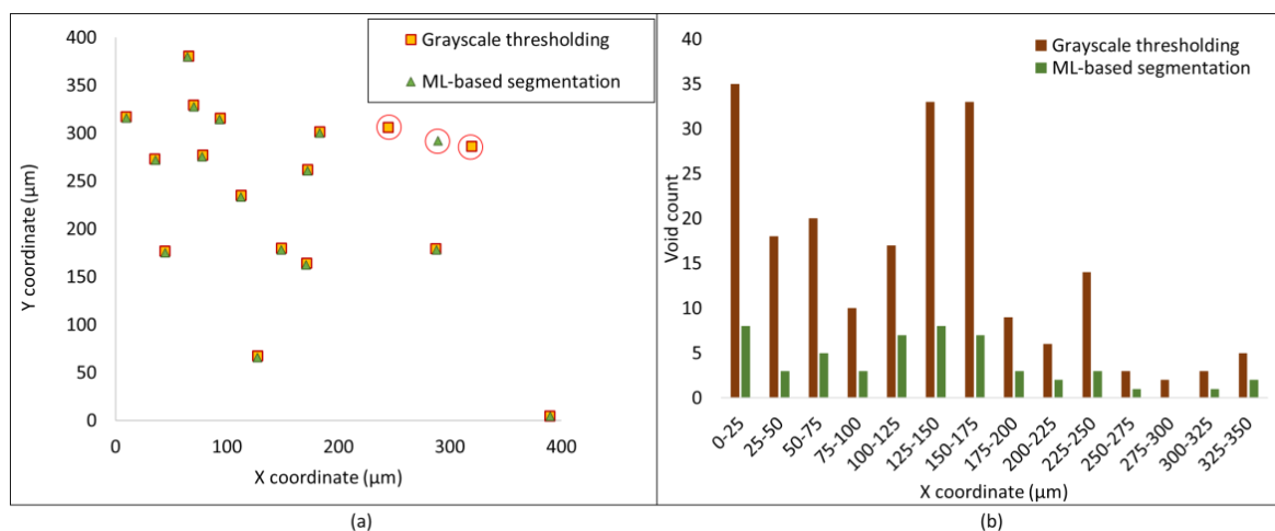
Figure 5: Comparison of void location (a) Centroid of each void in 2D slice (b) Void count along scan horizontal axis in 3D volume.
