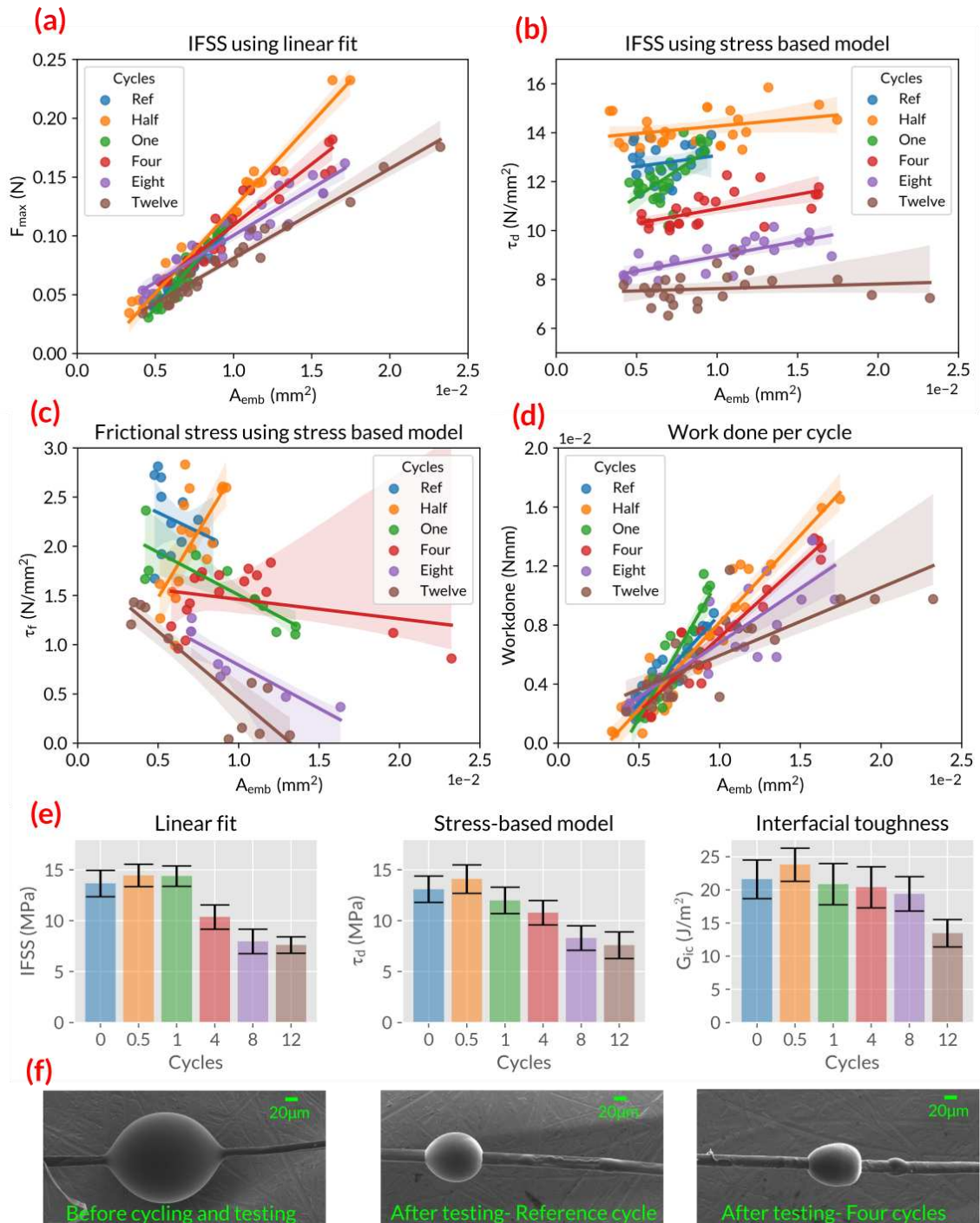
Figure 5. (a)-(d) Measurement results of MB test; (e) variation of IFSS, \tau_d and G_{ic} for different cycles; (f) SEM images of the droplets.
