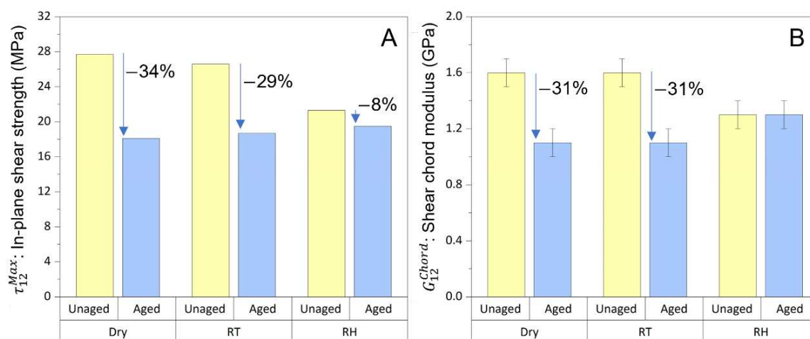
Figure 5. Effect of water immersion ageing on \tau_{12}^{Max} (A) and G_{12}^{Chord} (B) values of composites
