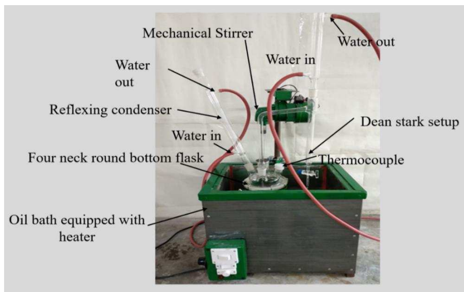
Figure 1 Recycling setup for waste PET.
