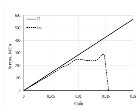
Figure 3. Tension stress – strain curve of FRP composite
