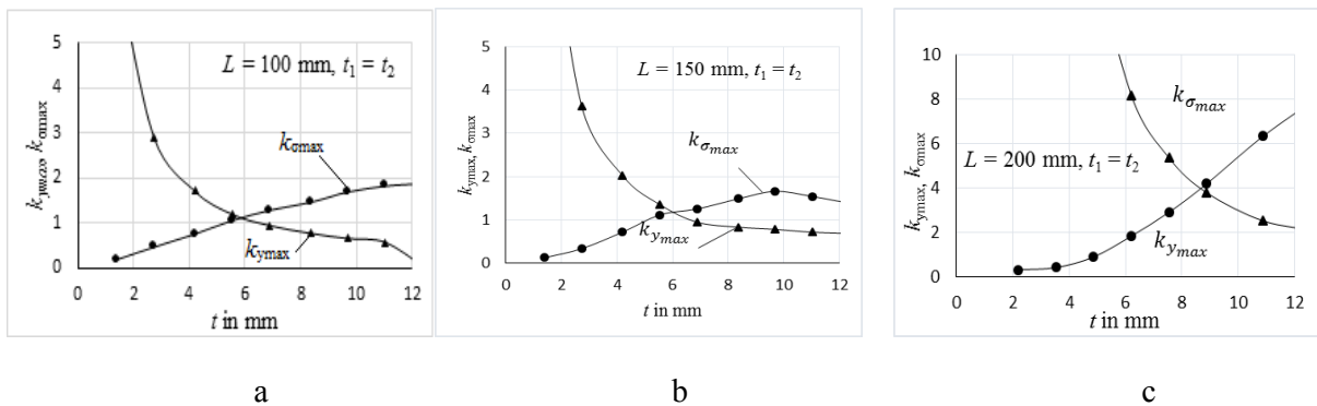
Figure 11. Influence of FRP Thickness t on coefficient k_{y_{max}} and k_{\sigma_{max}} . where the top facesheet thickness t_1 is equal to bottom face sheet t_2 lengths between supports respectively 100, 150, 200 mm.
