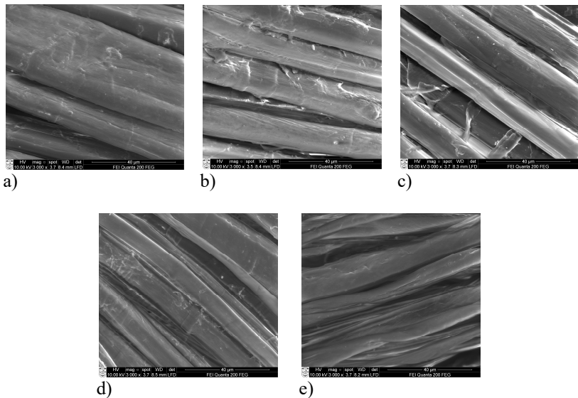
Figure 3. Surface view of terry fabrics, SEM pictures (40 µm): a) ramie fiber, b) unbleached flax fiber, c) bleached flax fiber, d) hemp fiber, e) cotton fiber
