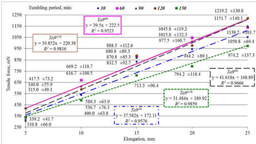
Figure 5. Dependence of tensile force parameter of terry fabrics variant Ta9^{30-150} on the pile loop pulling distance
