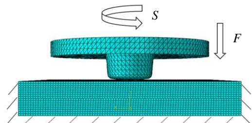
Fig. 7 Boundary conditions
