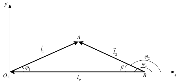
Fig. 2 Vector polygon of the four bar linkage with a sliding block constructed on the basis of kinematic chain OO_1AB
