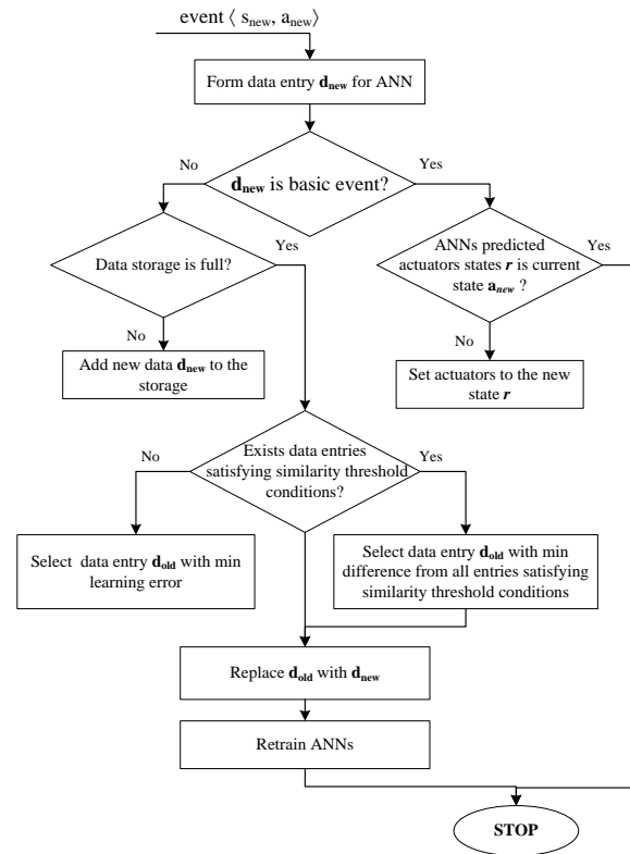
Figure 4. ANN Decision-Making Algorithm for Behaviour-Based Intelligent Control
