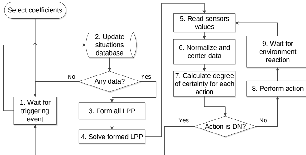
Figure 3. The intelligent light control algorithm based on augmenting self-training procedure (Fig. 2)
