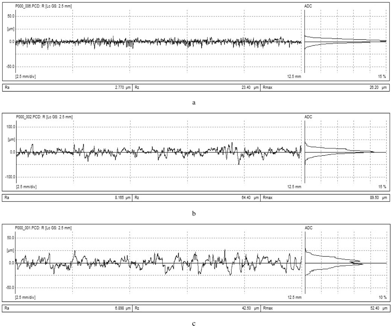
Fig. 1. Typical surface roughness R_z profiles of birch wood: a – along the wood grain; b – across the grain; c – in the angle of 45^\circ
