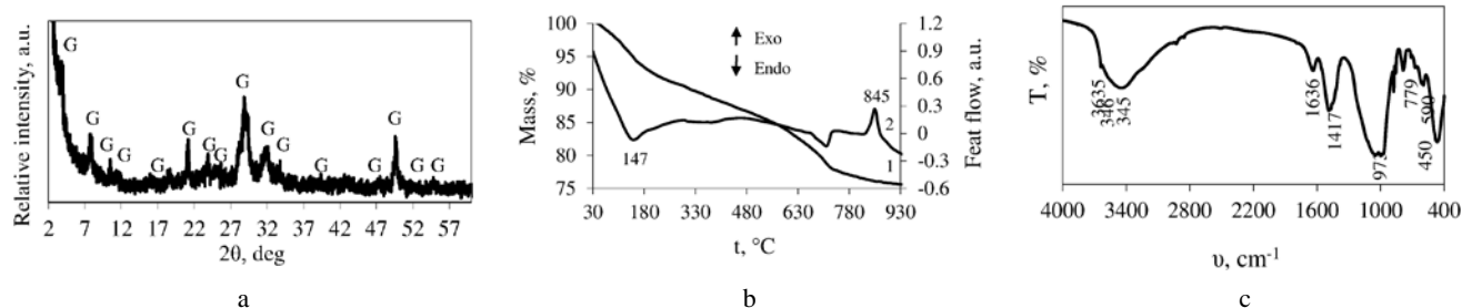
Fig. 6. X-ray diffraction pattern (a), DSC – TG curves (b) and FT-IR spectrum (c) of gyrolite substituted with Fe 3+ ions. Indexes: G – gyrolite
