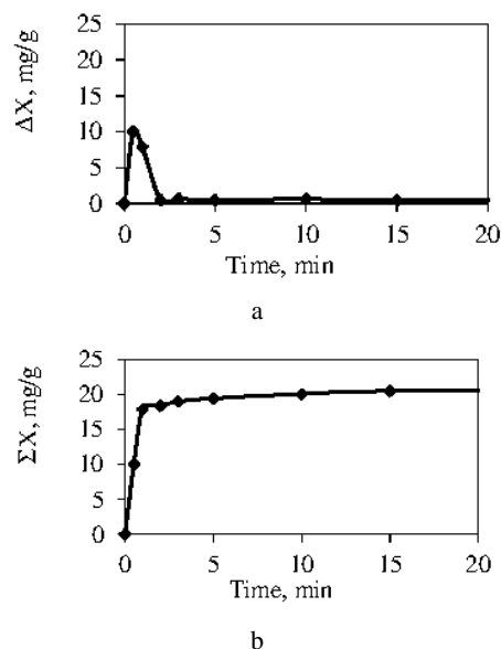
Fig. 1. Differential (a) and integral (b) kinetic curves of \text{Ni}^{2+} ions adsorption by gyrolite
