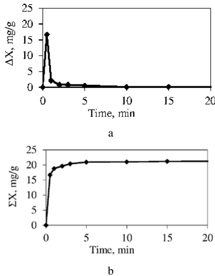
Fig. 2. Differential (a) and integral (b) kinetic curves of \text{Ca}^{2+} ions concentration variation in acidic solution
