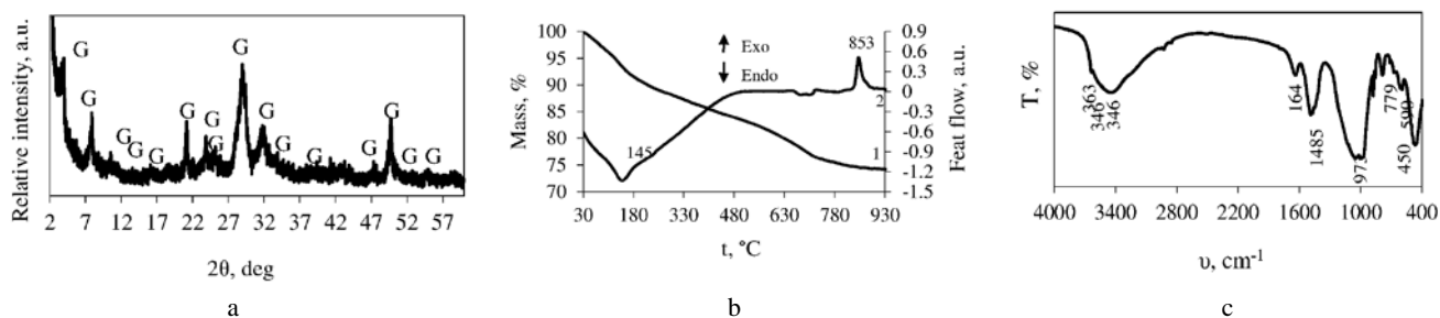
Fig. 5. X-ray diffraction pattern (a), DSC – TG curves (b) and FT-IR spectrum (c) of gyrolite. Duration of hydrothermal synthesis at 200 °C is 48 h. Indexes: G – gyrolite
