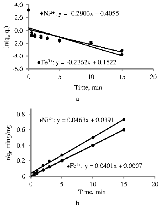
Fig. 4. Pseudo first-order (a) and pseudo-second order (b) kinetic plots in acidic solutions
